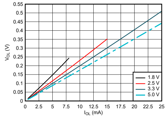
5-2. Output Voltage vs Current in LOW State
