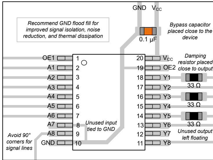
図 10-3. Example Layout for the SN74LV8T541-Q1 in TSSOP
