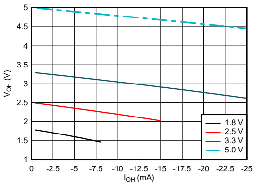
5-1. Output Voltage vs Current in HIGH State
