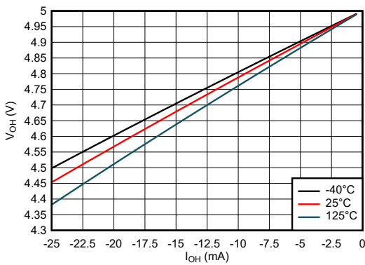
5-3. Output Voltage vs Current in HIGH State; 5-V Supply
