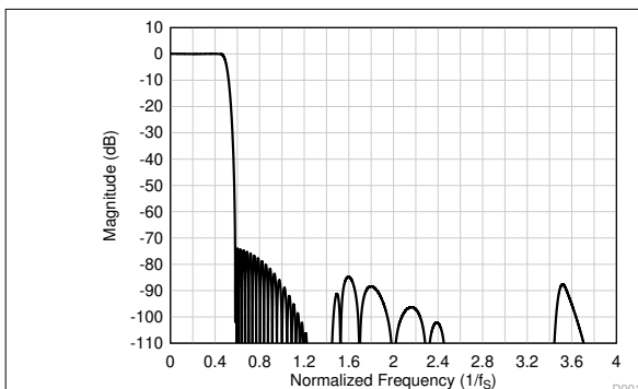
図 6-27. Linear Phase Decimation Filter Magnitude Response
