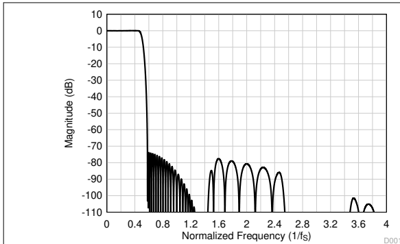
図 6-25. Linear Phase Decimation Filter Magnitude Response
