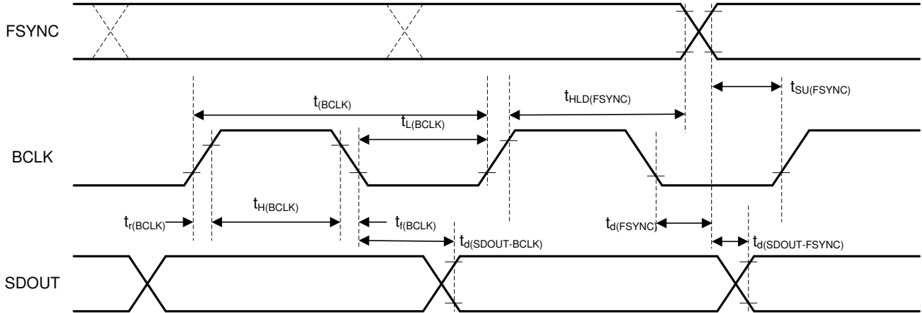
図 5-3. TDM (With BCLK_POL = 1), I 2 S, and LJ Interface Timing Diagram
