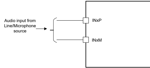
図 7-16. Differential DC-Coupled Input Connection (ADC_CHx_INSRC set to 2'b00 and ADC_CHx_CM_TOL set to 2'b01 or 2'10)
