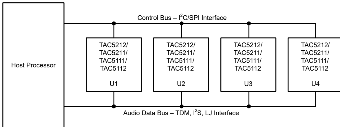
图 7-14. Multiple TAC5211 Devices With Shared Control and Audio Data Buses
