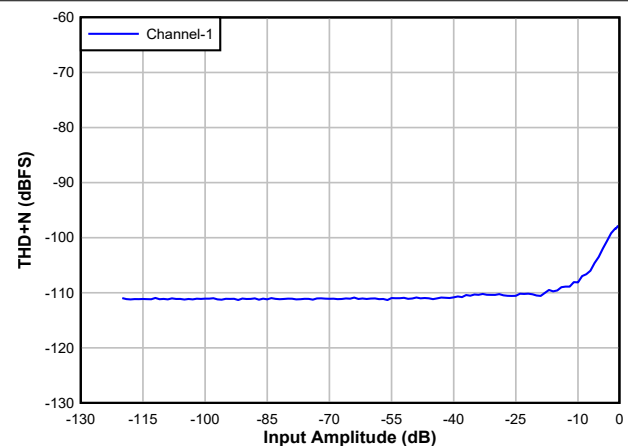
6-6. ADC THD+N Level vs Input
