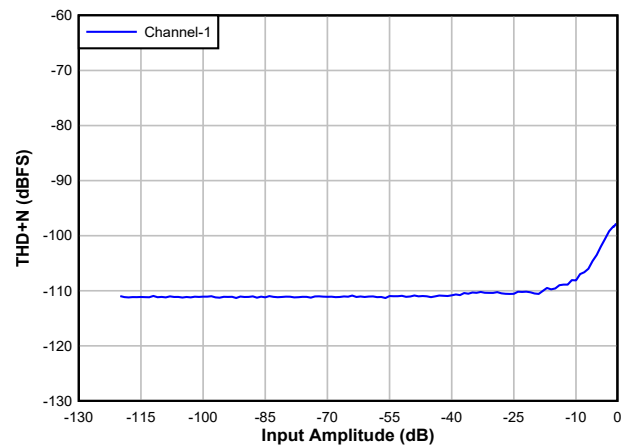
6-6. ADC THD+N Level vs Input
