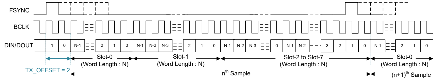
7-4. TDM Mode Protocol Timing (No Idle BCLK Cycles, PASI_TX_OFFSET = 2)
