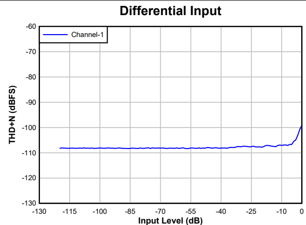
6-6. ADC THD+N Level vs Input
