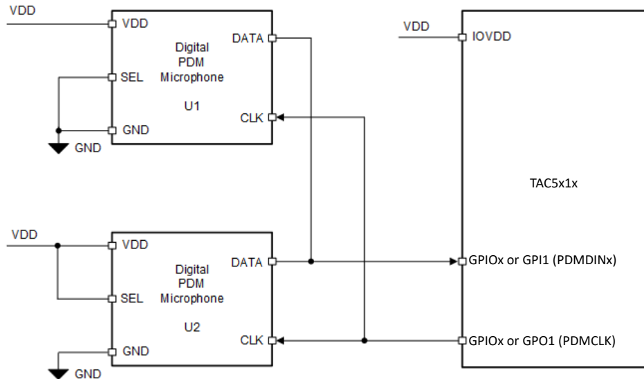
7-25. Digital PDM Microphones Connection Diagram for the TAC5211
