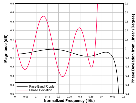
図 7-94. Low-latency Interpolation Filter Pass-Band Ripple and Phase Deviation
