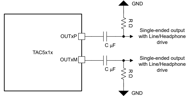
7-24. Stereo Single-ended Output Connection (OUT1x_CFG[2:0] = 3'b001)
