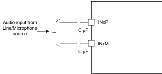
図 7-15. Differential AC-Coupled Input Connection (ADC_CHx_INSRC set to 2'b00 and ADC_CHx_CM_TOL set to 2'b00 or 2'b01 or 2'10)
