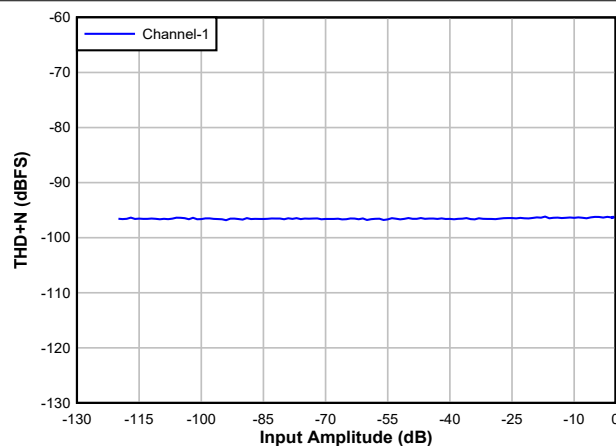
6-5. ADC THD+N Level vs Input
