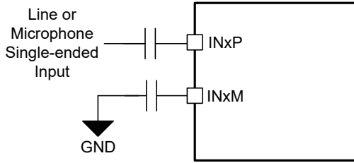
図 7-17. Single-ended AC-Coupled Input Connection (ADC_CHx_INSRC set to 2'b01 and ADC_CHx_CM_TOL set to 2'b00 or 2'b01 or 2'10)
