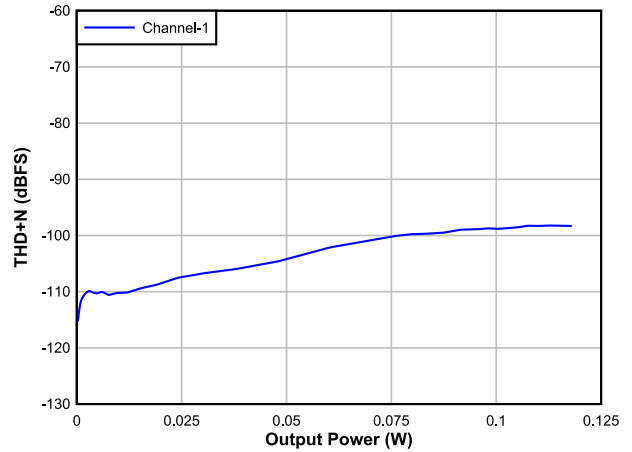
6-22. DAC THD+N Level vs output power
