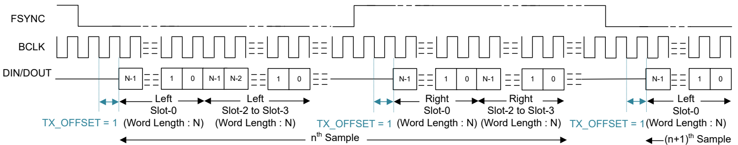
6-7. I 2 S Protocol Timing (PASI_TX_OFFSET = 1)
