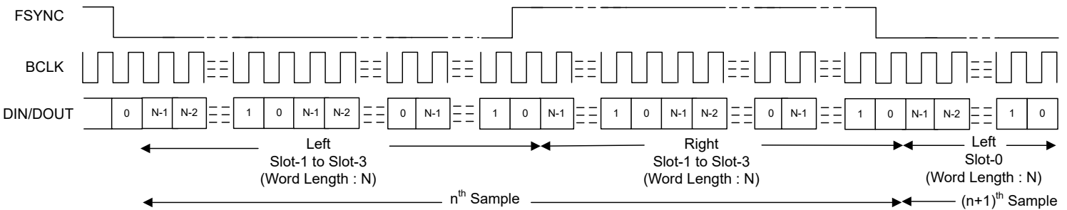
6-8. I 2 S Protocol Timing (No Idle BCLK Cycles, PASI_TX_OFFSET = 0)
