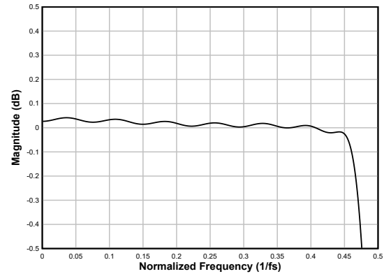
図 6-66. Linear-phase Decimation Filter Pass-Band Ripple
