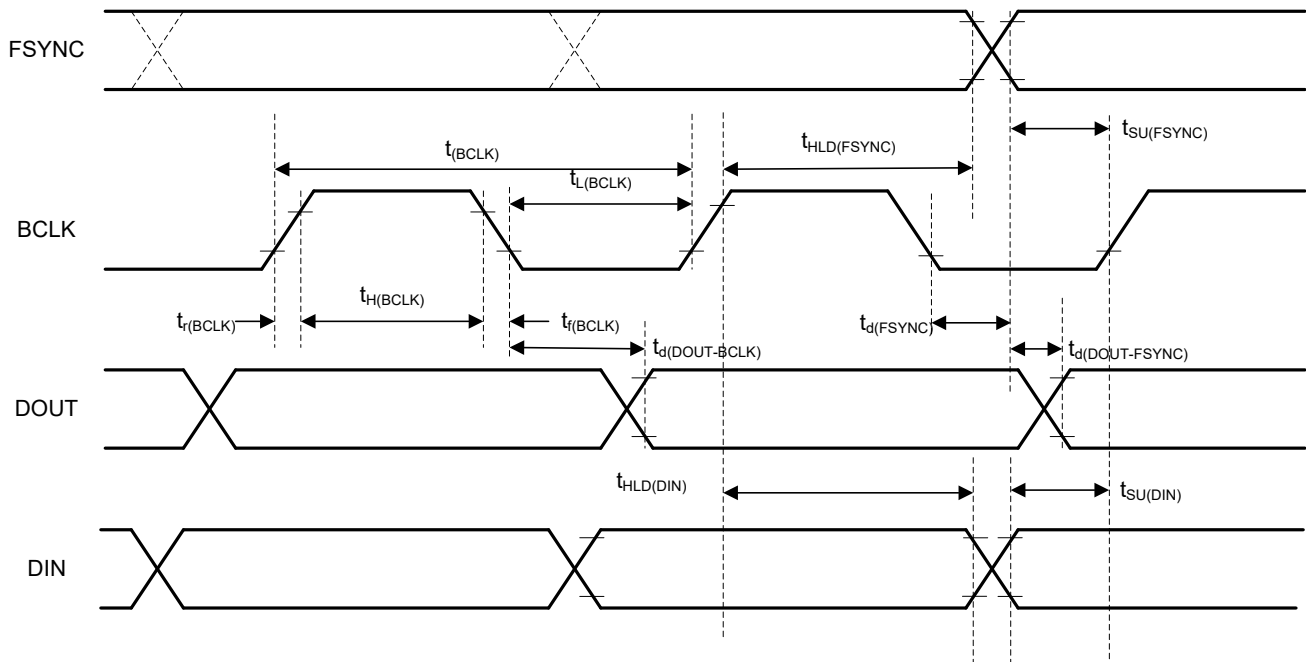
図 5-3. TDM (With BCLK_POL = 1), I²S, and LJ Interface Timing Diagram
