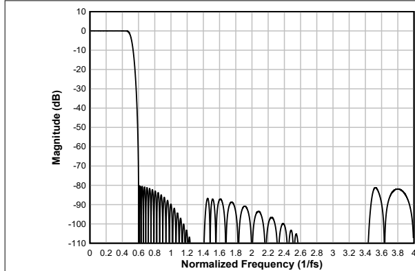
図 6-65. Linear-phase Decimation Filter Magnitude Response
