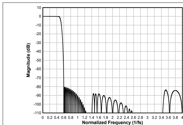
図 6-22. Linear-phase Interpolation Filter Magnitude Response
