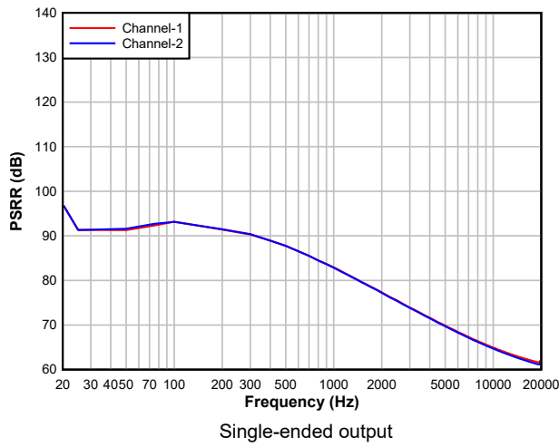
5-19. DAC PSRR vs Frequency
