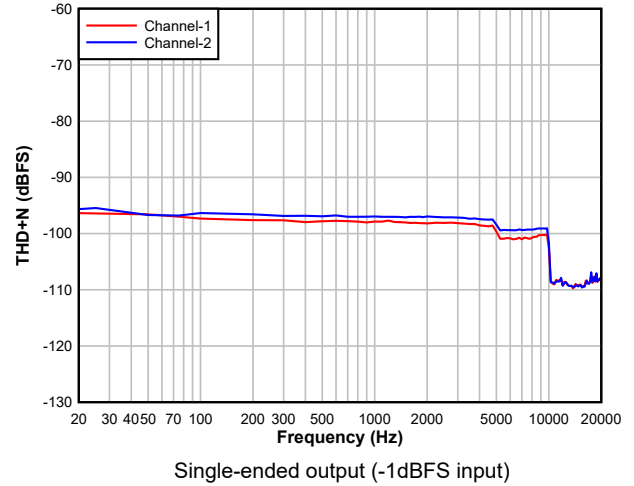
5-12. DAC THD+N Level vs Frequency
