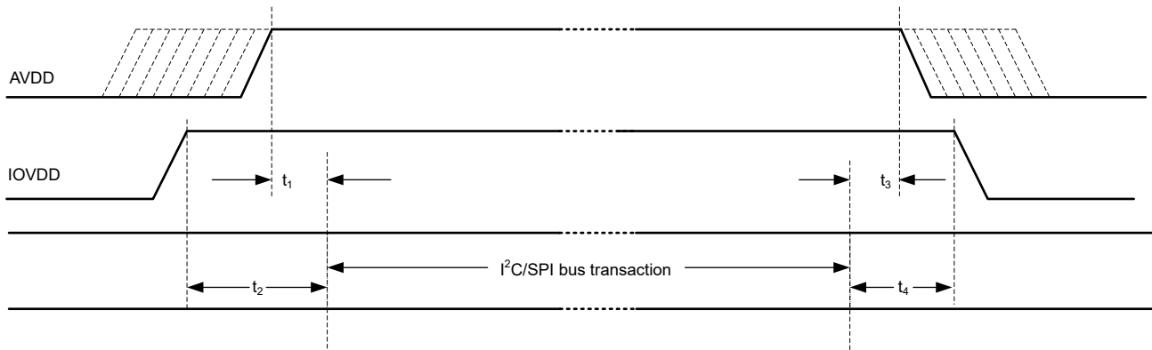
図 8-4. Power-Supply Sequencing Requirement Timing Diagram
