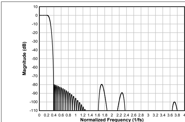
図 6-76. Linear-phase Decimation Filter Magnitude Response
