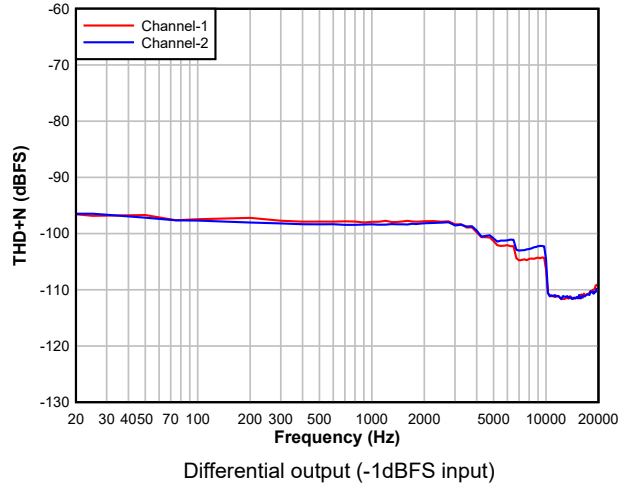
5-11. DAC THD+N Level vs Frequency
