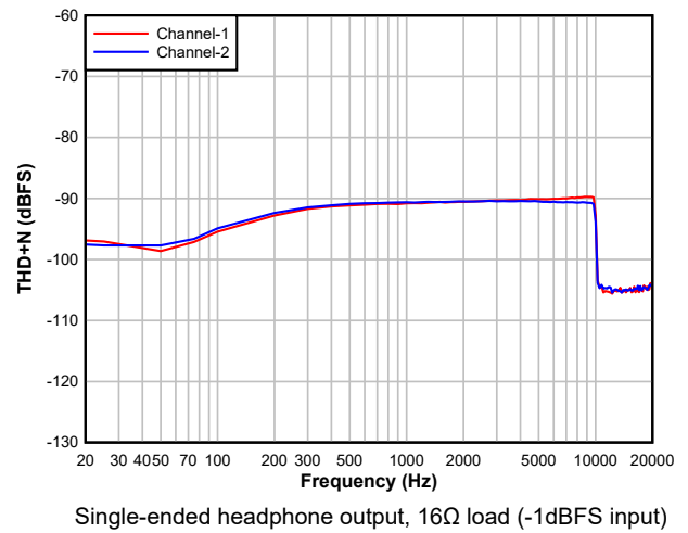
5-14. DAC THD+N Level vs Frequency
