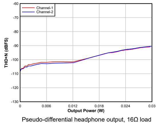
5-10. DAC THD+N Level vs output power
