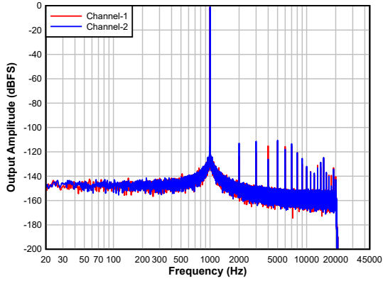
5-17. DAC FFT with -1dBFS Input
