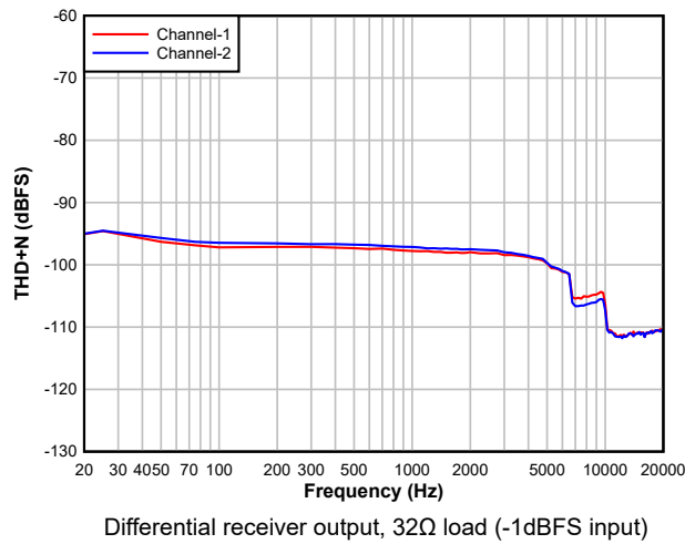
5-13. DAC THD+N Level vs Frequency
