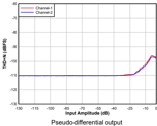
5-7. DAC THD+N Level vs Input
