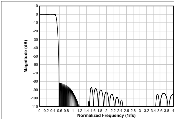
図 6-26. Linear-phase Interpolation Filter Magnitude Response
