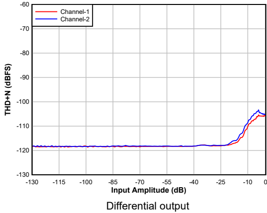
5-5. DAC THD+N Level vs Input
