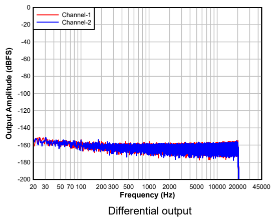
5-15. DAC FFT with Idle Channel Input
