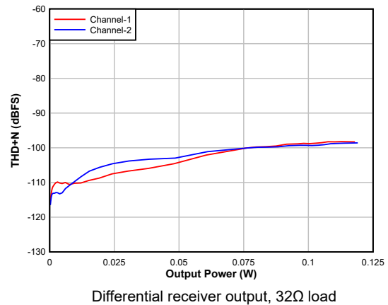
5-8. DAC THD+N Level vs output power
