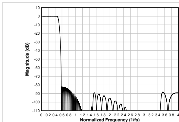
図 6-30. Linear-phase Interpolation Filter Magnitude Response
