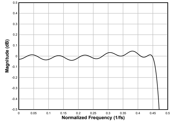
図 6-69. Linear-phase Decimation Filter Pass-Band Ripple
