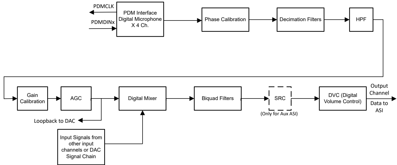
❏ 6-60. PDM Recording Signal-Chain Processing Flowchart
