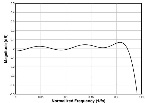
図 6-77. Linear-phase Decimation Filter Pass-Band Ripple
