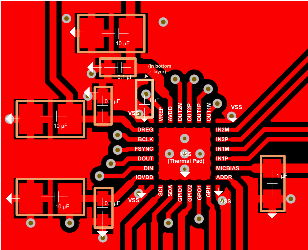
8-5. Example Layout
