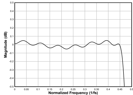
図 6-71. Linear-phase Decimation Filter Pass-Band Ripple
