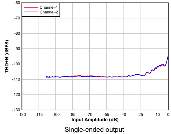
5-6. DAC THD+N Level vs Input
