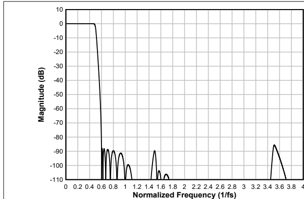
図 6-96. Ultra Low-latency Decimation Filter Magnitude Response
