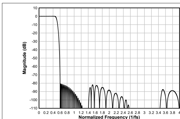
図 6-66. Linear-phase Decimation Filter Magnitude Response
