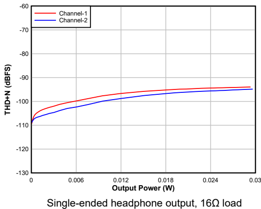
5-9. DAC THD+N Level vs output power
