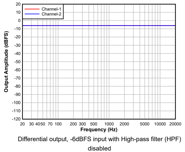
5-20. DAC Frequency Response
