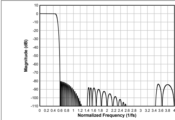
図 6-24. Linear-phase Interpolation Filter Magnitude Response
