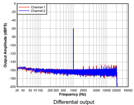
5-16. DAC FFT with -60dBFS Input
