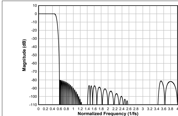
図 6-64. Linear-phase Decimation Filter Magnitude Response
