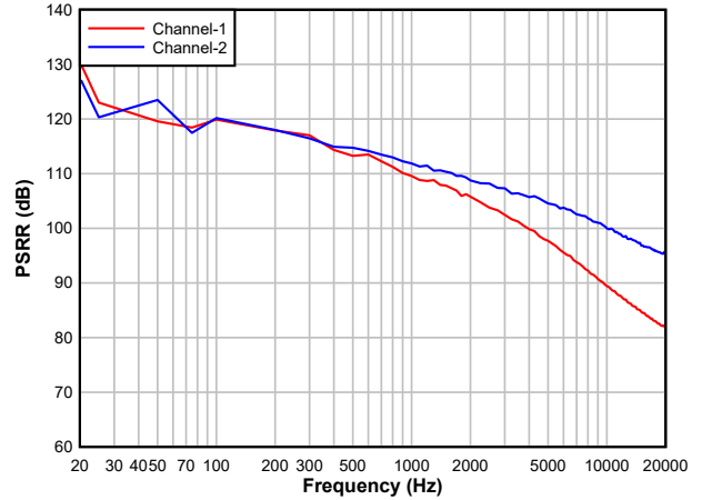
5-18. DAC PSRR vs Frequency
