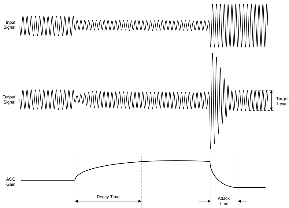
Figure 6-100. AGC Characteristics
