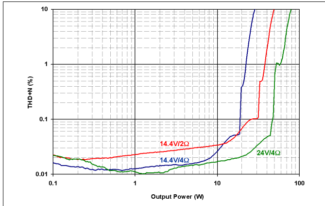
Figure 3. THD+N vs BTL Output Power at 1kHz
