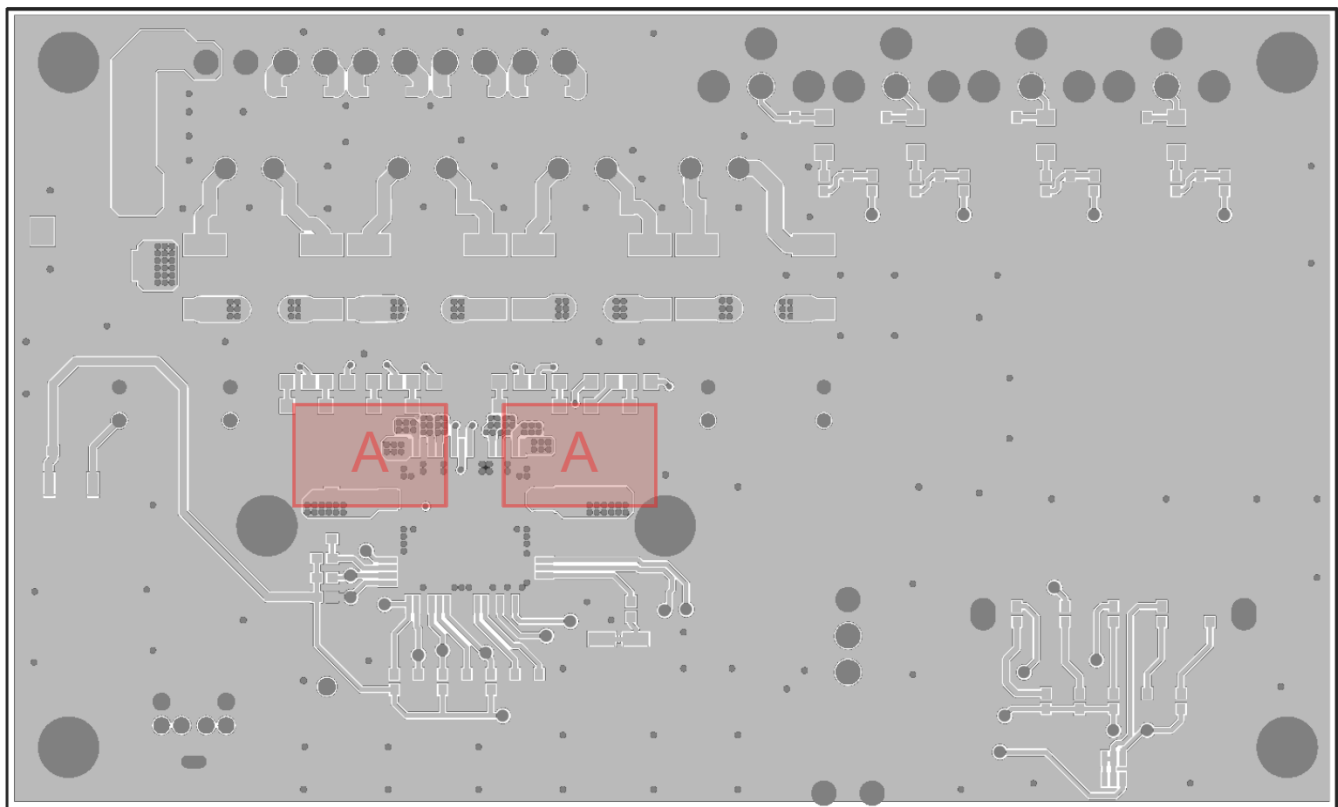
Figure 39. Top Layer
