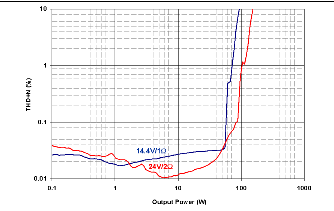
Figure 4. THD+N vs PBTB Output Power at 1kHz
