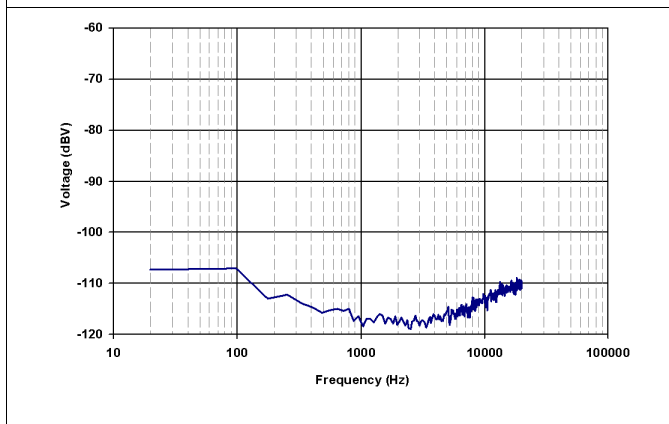
Figure 7. Noise FFT
