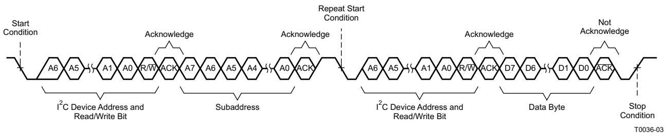
7-6. Random Read Transfer
