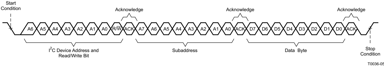
7-5. Random Write Transfer
