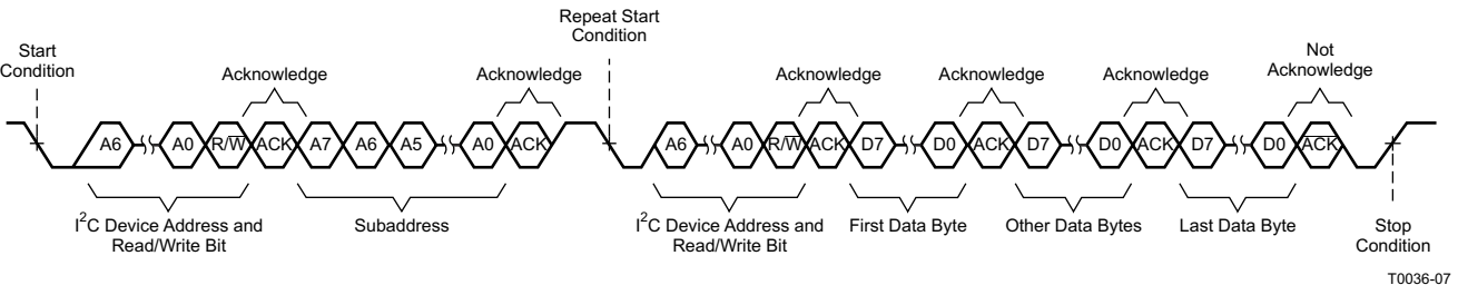
7-7. Sequential Read Transfer
