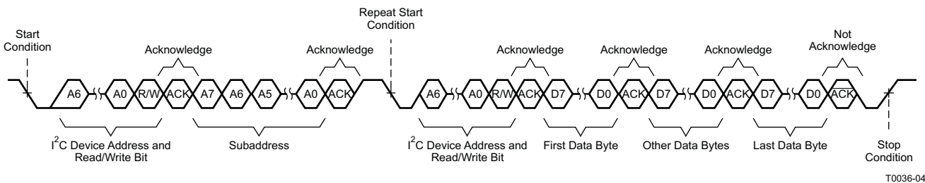
Figure 54. Multiple-Byte Read Transfer
