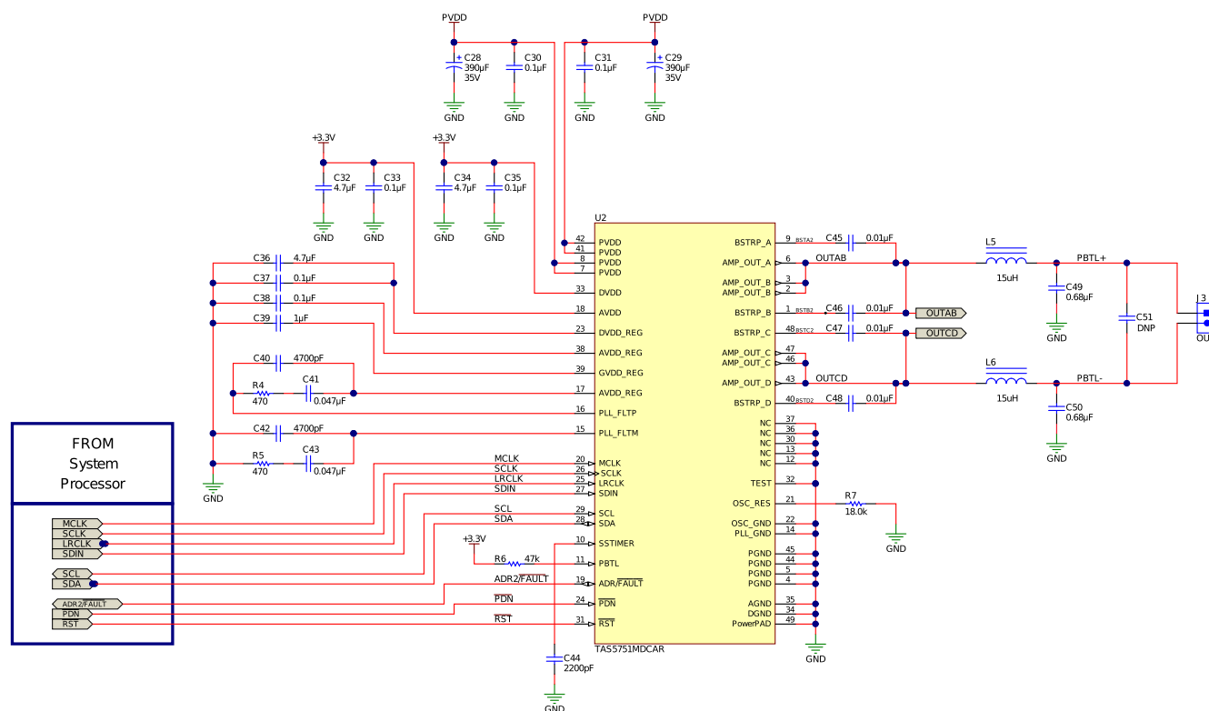
69. Mono Parallel Bridge Tied Load Application
