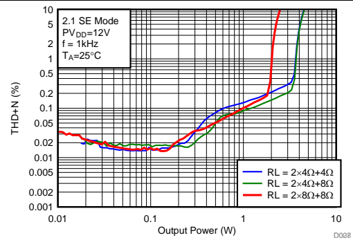
FIG 6. Total Harmonic Distortion + Noise vs Output Power
