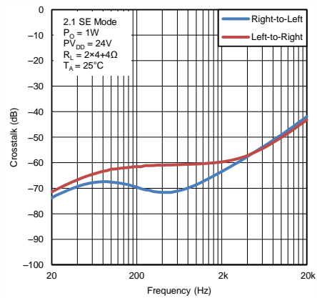
17. Crosstalk vs Frequency
