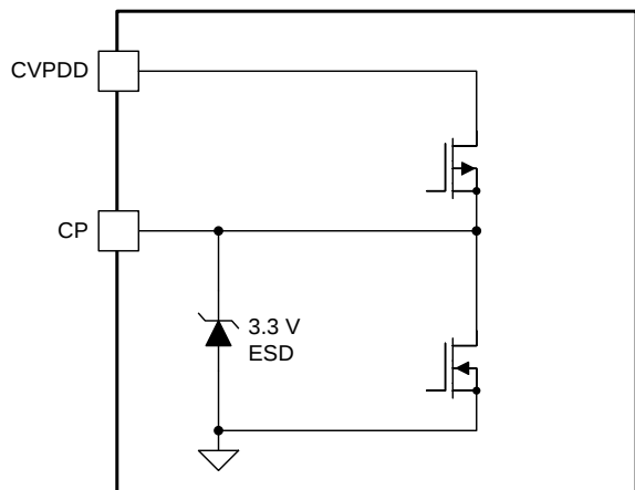
Figure 13. CP Pin
