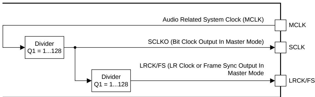
Figure 58. Simplified Clock Tree for MCLK Sourced Master Mode
