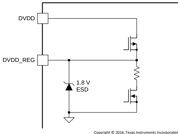
Figure 15. DVDD_REG Pin
