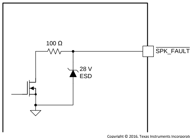
Figure 16. \overline{\text{SPK\_FAULT}} Pin
