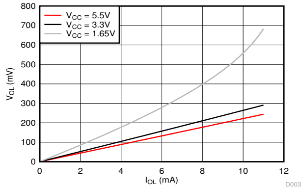
図 5-1. SDA Output Low Voltage ( V_{OL} ) vs Load Current ( I_{OL} ) at Three V_{CC} Levels ( T_A = 25^\circ\text{C} )
