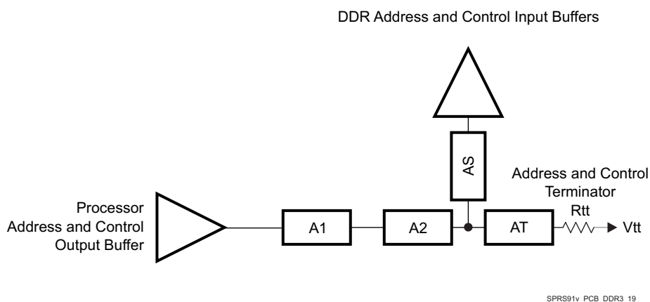
8-62. ADDR_CTRL Topology for One DDR3 Device
