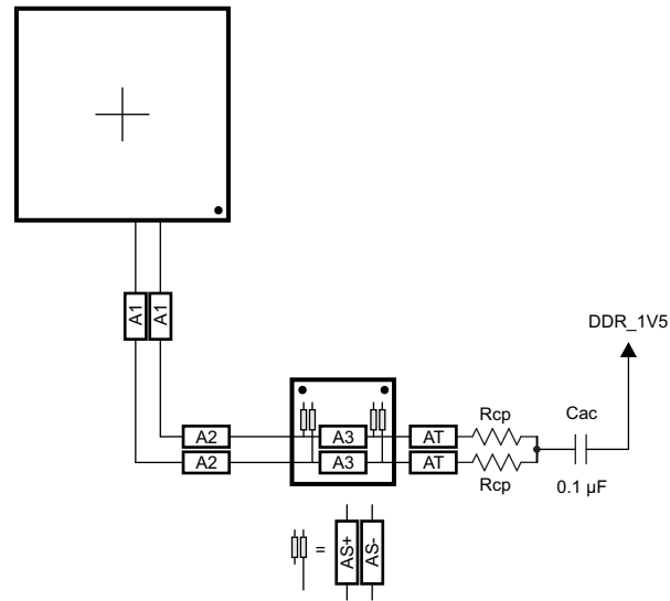
✎ 8-59. CK Routing for Two Mirrored DDR3 Devices
