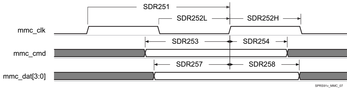
図 7-45. MMC/SD/SDIOj in - SDR25 - Receiver Mode
