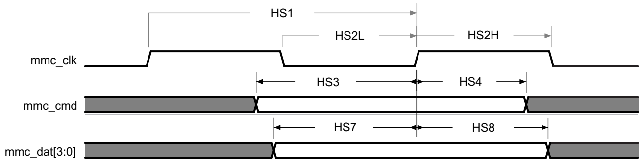
図 7-41. MMC/SD/SDIOj in - High Speed - Receiver Mode
