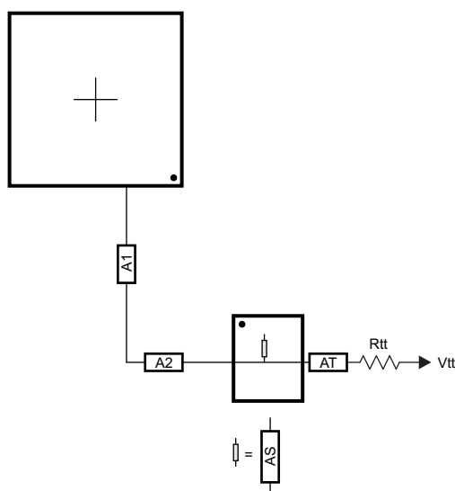
8-63. CK Routing for One DDR3 Device
