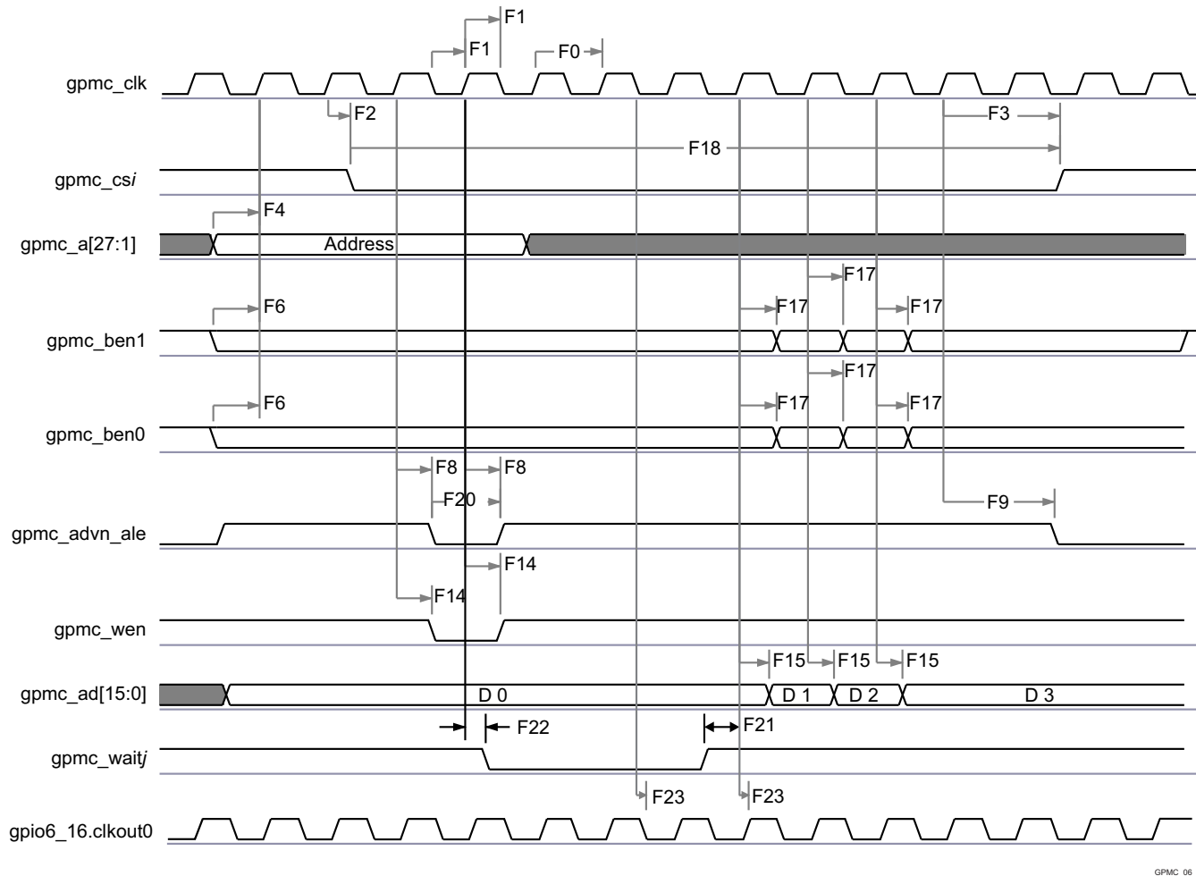
☒ 7-12. GPMC / Non-Multiplexed 16bits NOR Flash - Synchronous Burst Write 4x16bits - (GpmcFCLKDivider = 0) (1)(2)
