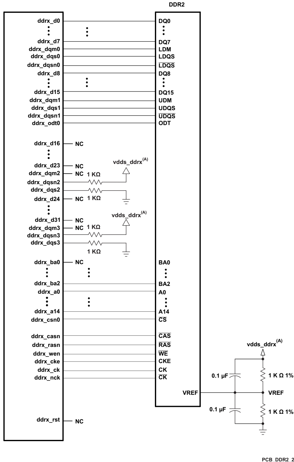
8-39. 16-Bit DDR2 High-Level Schematic
