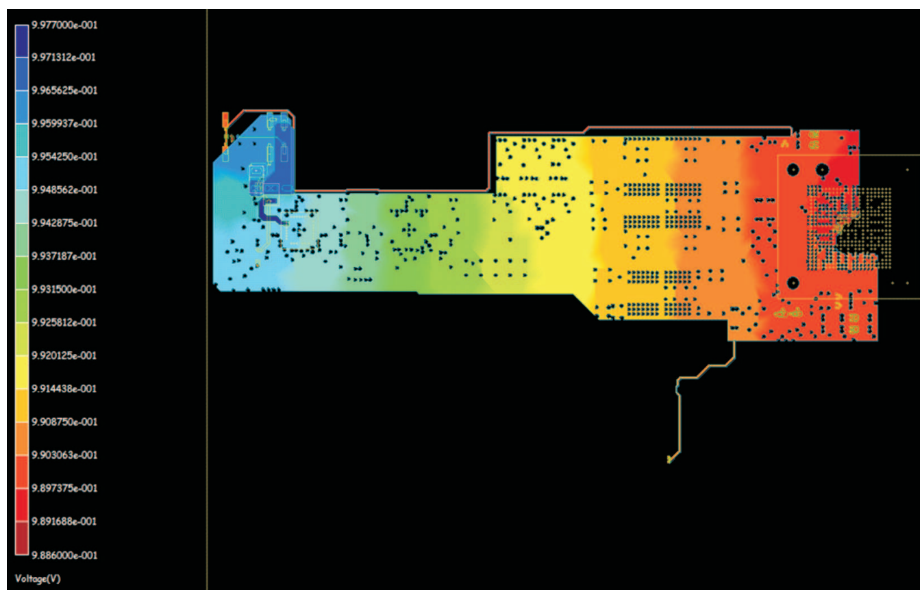
図 8-16. vdd_dspeve Voltage/IR Drop [All Layers]
