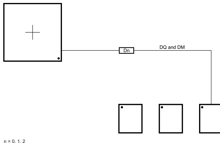
❏ 8-68. DQ/DM Routing With Any Number of Allowed DDR3 Devices
