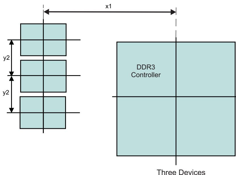
图 8-47. Placement Specifications
