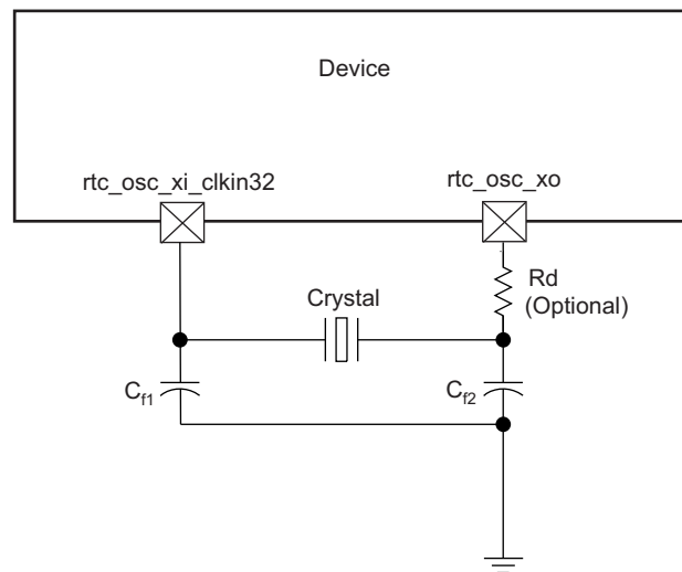
8-21. Grounding Scheme for Low-Frequency Clock
