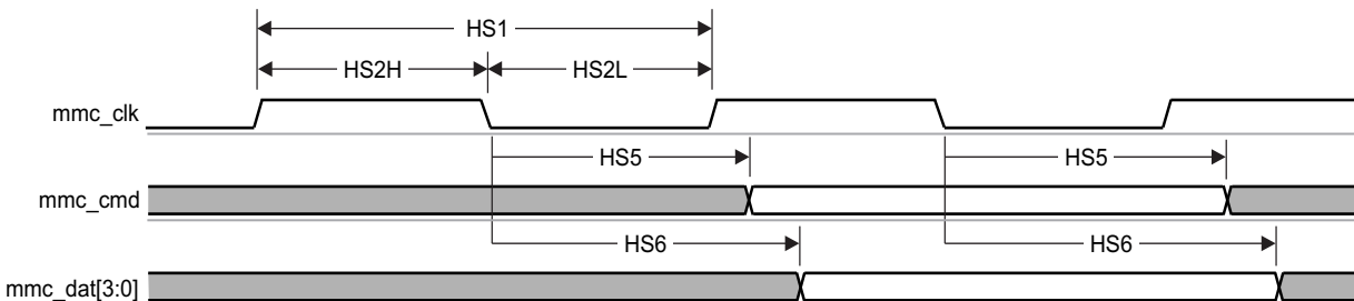
図 7-42. MMC/SD/SDIOj in - High Speed - Transmitter Mode
