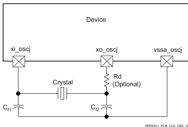
图 8-22. Grounding Scheme for High-Frequency Clock
