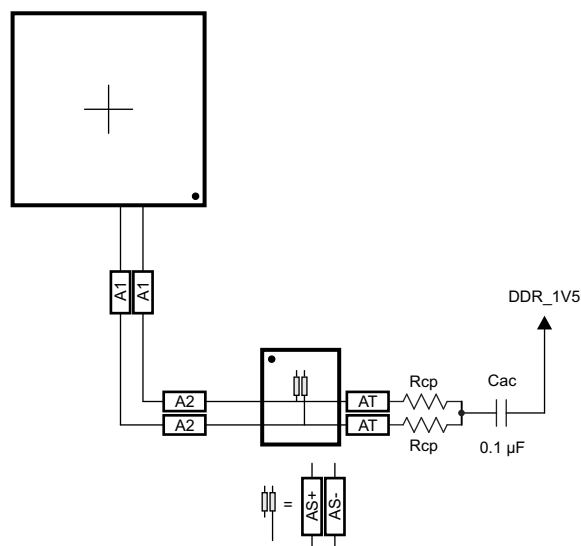
8-63. CK Routing for One DDR3 Device
