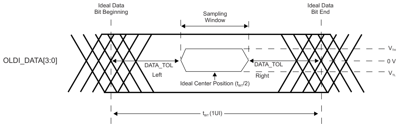
7-107. OLDI Data Output Jitter
