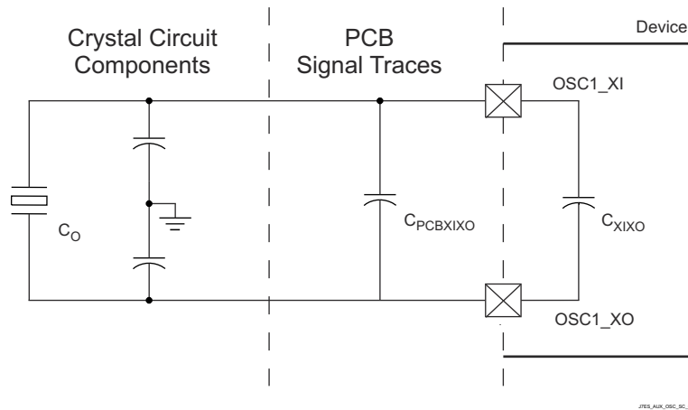
图 7-31. Shunt Capacitance
