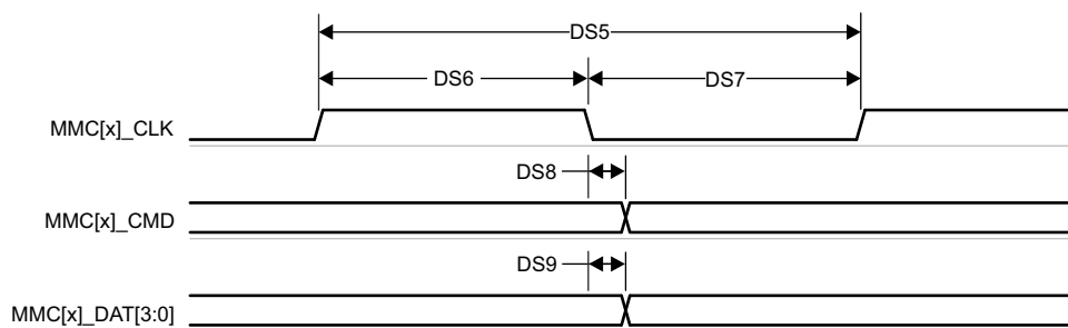
图 7-86. MMC1/2 – Default Speed – Transmit Mode
