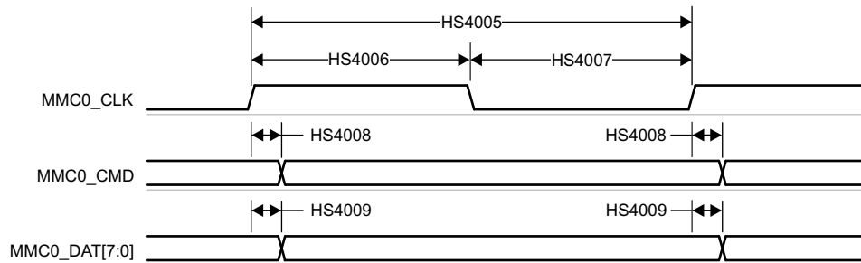
図 7-84. eMMC in – HS400 Mode – Transmitter Mode
