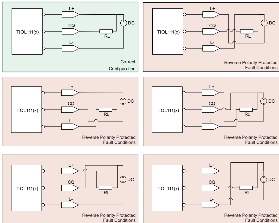
15. Low-Side Driver Configuration
