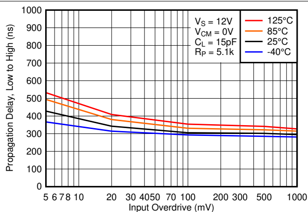
FIG 5-28. Low to High Propagation Delay vs. Input Overdrive Voltage, 12V
