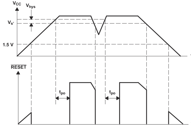
Figure 8-2. V_{CC} -RESET Response
