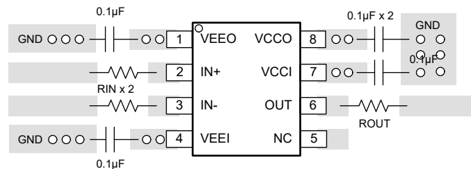
Figure 7-5. Layout Example
