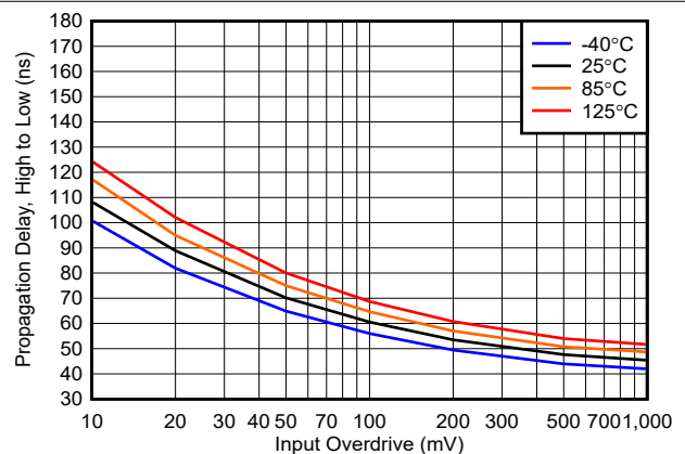
5-24. Propagation Delay, (High to Low) vs. Input Overdrive, 12V
