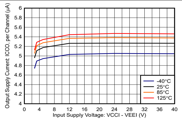
5-14. Output Supply Current vs. Input Supply Voltage, Output Low, No Load
