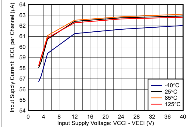
5-15. Input Supply Current vs. Input Supply Voltage, Output High, No Load
