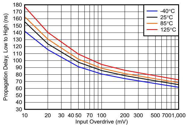
5-21. Propagation Delay, (Low to High) vs. Input Overdrive, 3.3V
