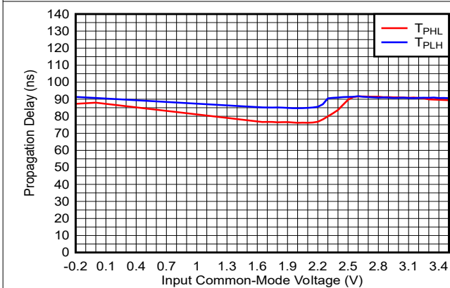
5-17. Propagation Delay vs. Common-Mode, 3.3V
