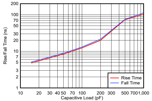
5-20. Rise/Fall Time vs. Capacitive Load, 12V
