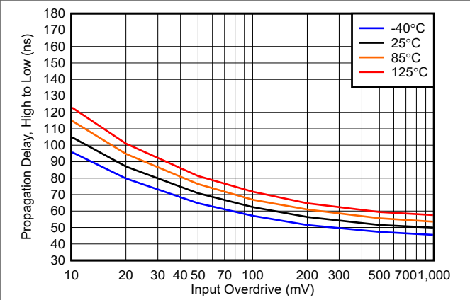
5-26. Propagation Delay, (High to Low) vs. Input Overdrive, 40V
