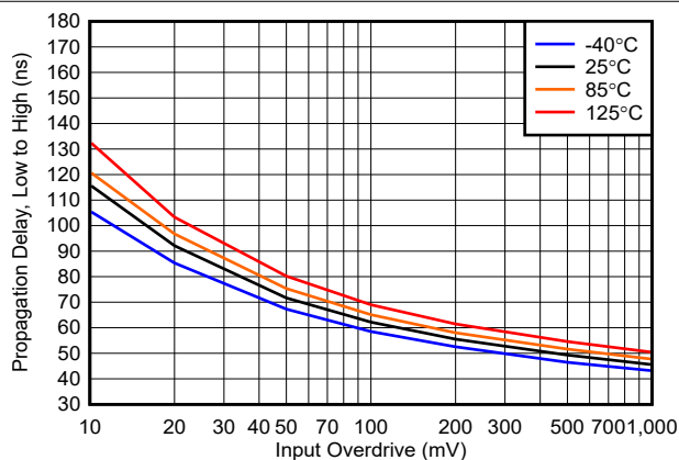
5-23. Propagation Delay, (Low to High) vs. Input Overdrive, 12V
