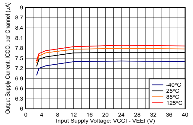
5-16. Output Supply Current vs. Input Supply Voltage, Output High, No Load
