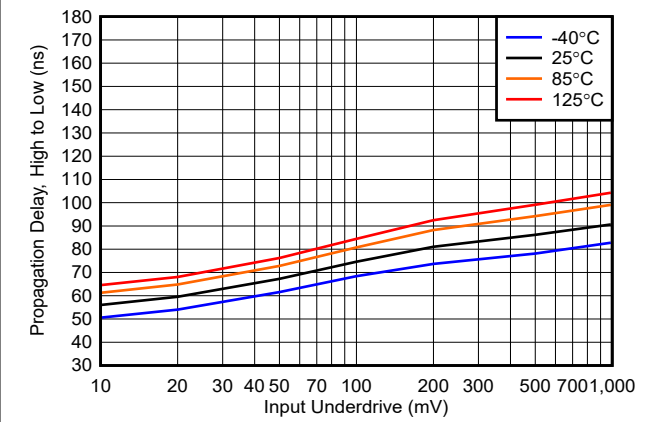
5-28. Propagation Delay, (High to Low) vs. Input Underdrive, 3.3V
