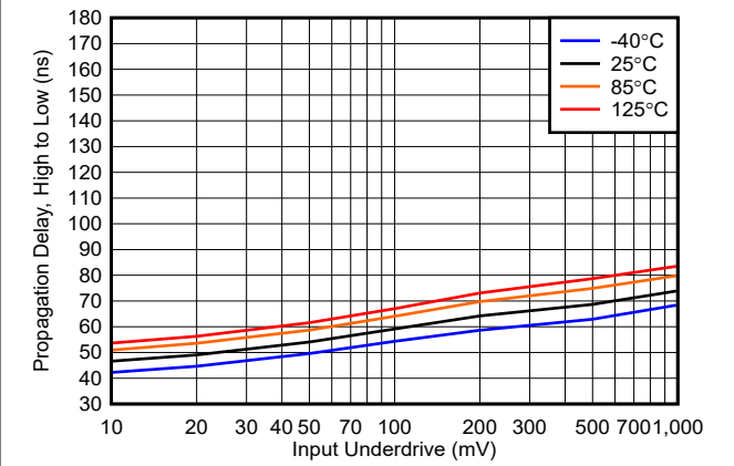
5-30. Propagation Delay, (High to Low) vs. Input Underdrive, 12V
