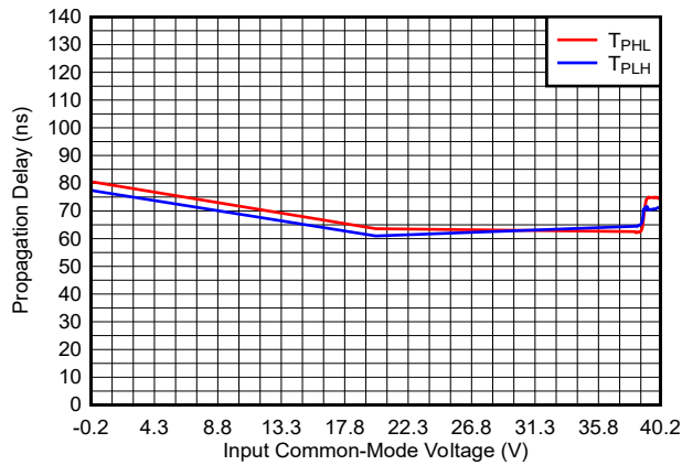
5-19. Propagation Delay vs. Common-Mode, 40V
