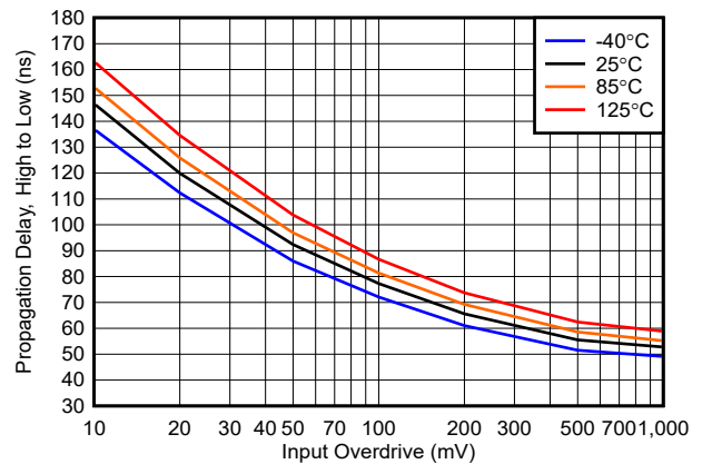
5-22. Propagation Delay, (High to Low) vs. Input Overdrive, 3.3V
