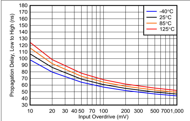
5-25. Propagation Delay, (Low to High) vs. Input Overdrive, 40V
