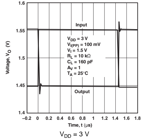
FIG 46. Inverting Small Signal
