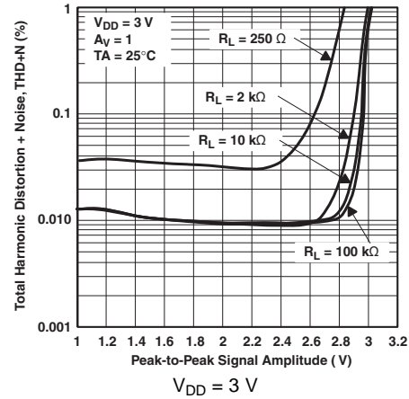
34. Total Harmonic Distortion Plus Noise vs Peak-to-Peak Signal Amplitude
