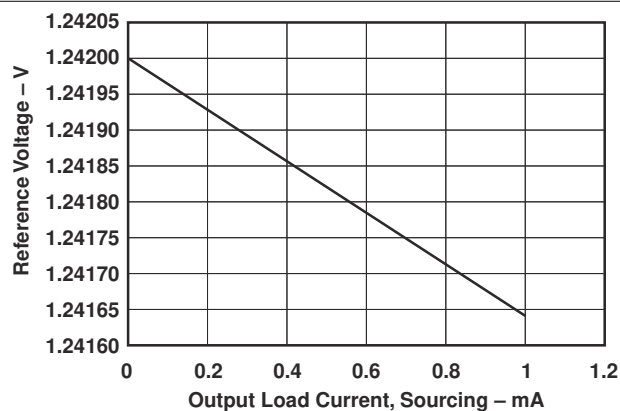
FIG 7-16. Reference Voltage vs Output Load Current (Sourcing)
