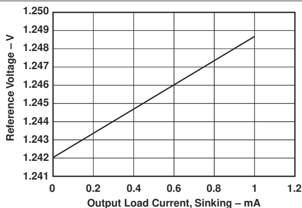
FIG 7-17. Reference Voltage vs Output Load Current (Sinking)
