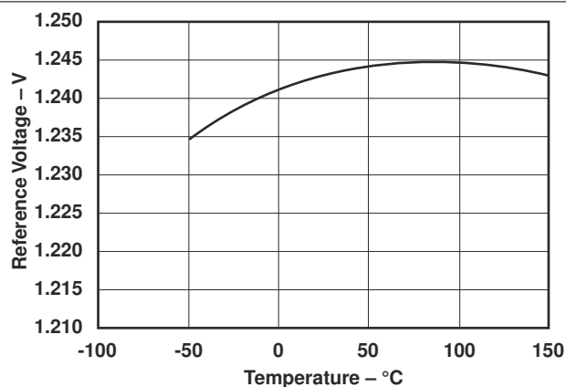
FIG 7-18. Reference Voltage vs Temperature
