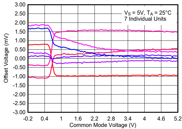
8-31. Offset Voltage vs. Common Mode Voltage, 5 V
