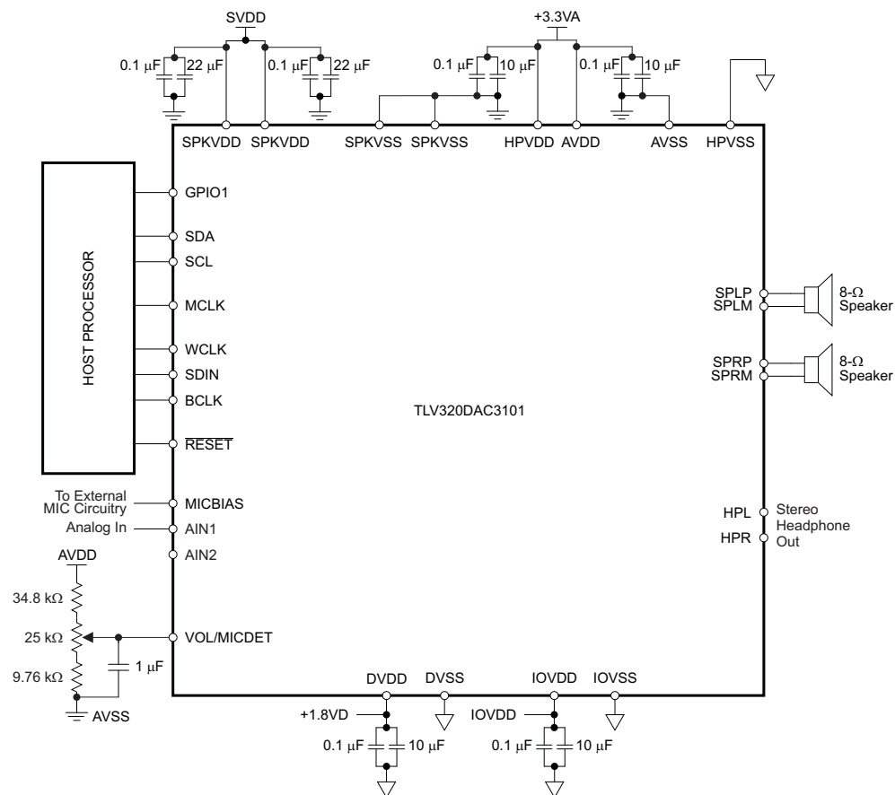
☒ 7-1. Typical Circuit Configuration
