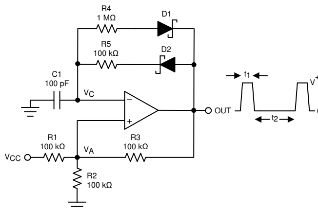
8-12. Adjustable Pulse Width Generator
