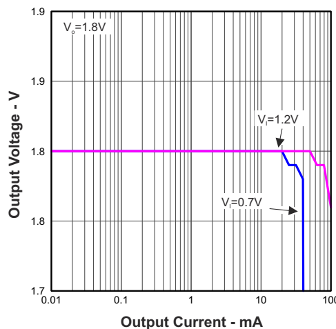
図 6-10. Output Voltage vs Output Current and Input Voltage
