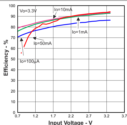
図 6-8. Efficiency vs Input Voltage and Output Current
