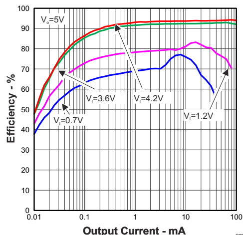
図 6-6. Efficiency vs Input Voltage and Output Current
