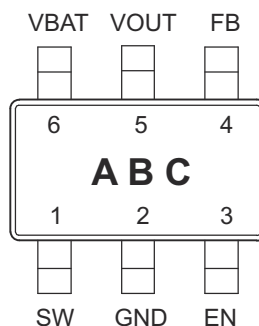
5-1. DBV Package 6 Pins Top View
