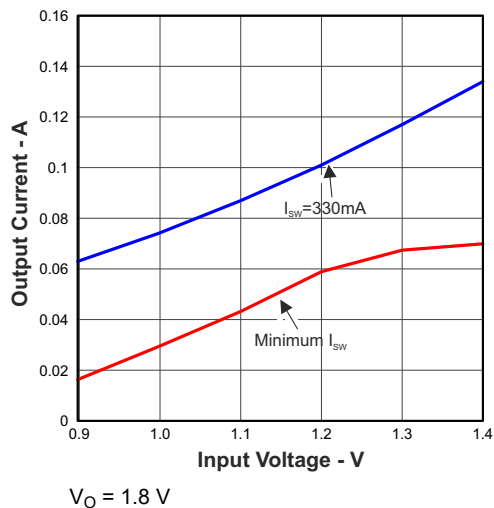
図 6-1. Maximum Output Current vs Input Voltage
