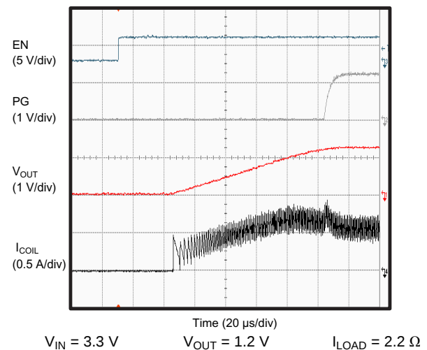
Figure 16. Startup
