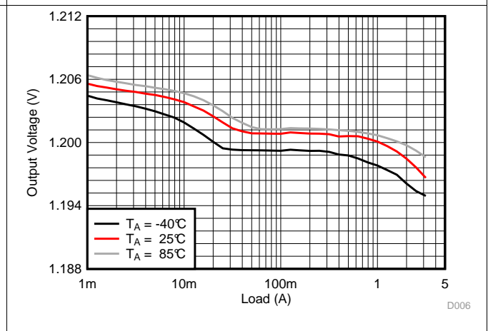
Figure 10. Load Regulation
