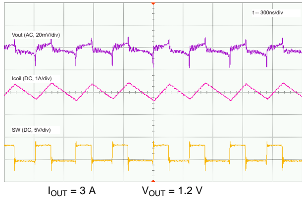
FIG 11. PWM Operation
