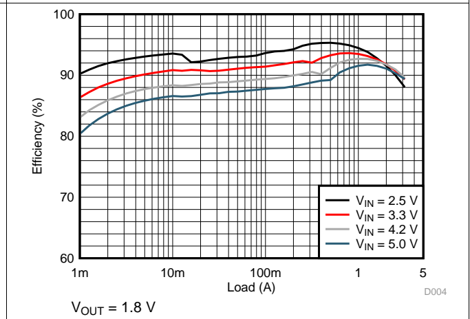
Figure 8. Efficiency
