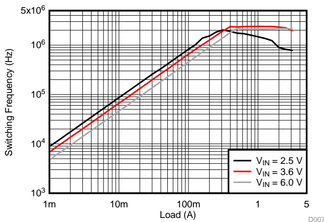
Fig 1. Switching Frequency
