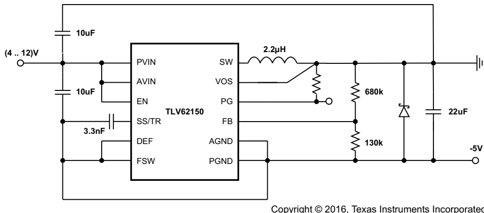
Figure 38. -5-V Inverting Power Supply
