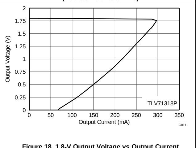
Figure 18. 1.8-V Output Voltage vs Output Current (Foldback Current Limit)
