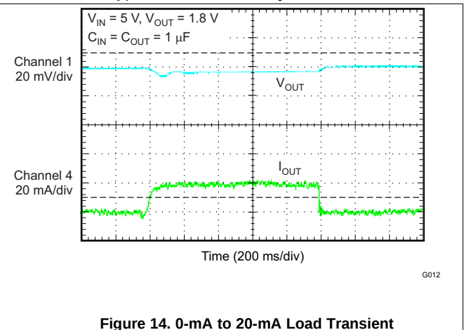
Figure 14. 0-mA to 20-mA Load Transient
