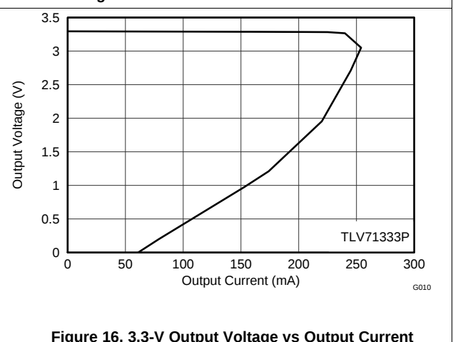
Figure 16. 3.3-V Output Voltage vs Output Current (Foldback Current Limit)
