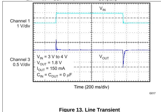
Figure 13. Line Transient
