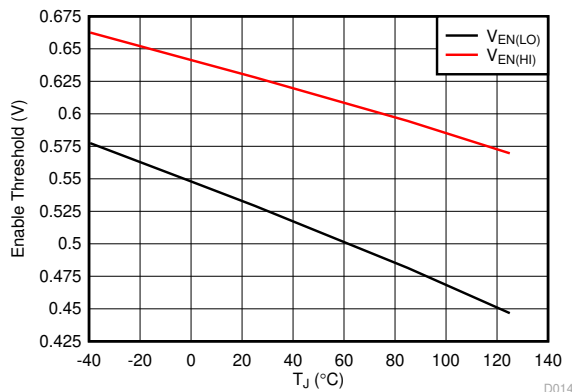
6-5. Enable Threshold vs Temperature
