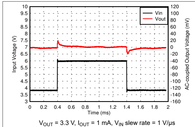
5-19. 3.3-V Line Transient
