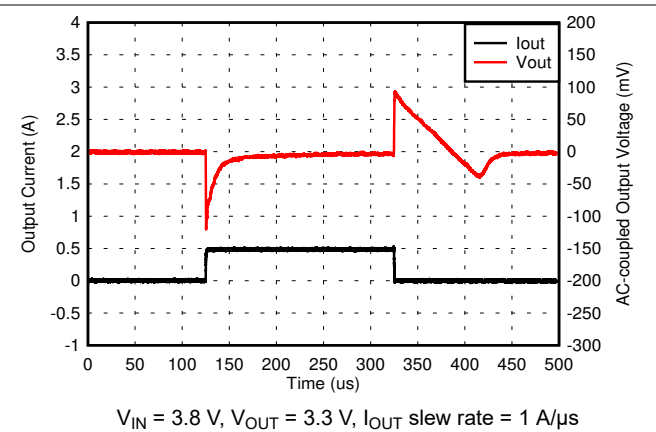
5-20. 3.3-V, 1-mA to 500-mA Load Transient
