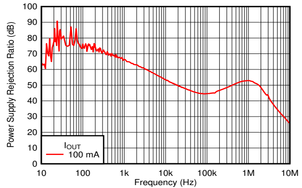
8-4. PSRR Performance
