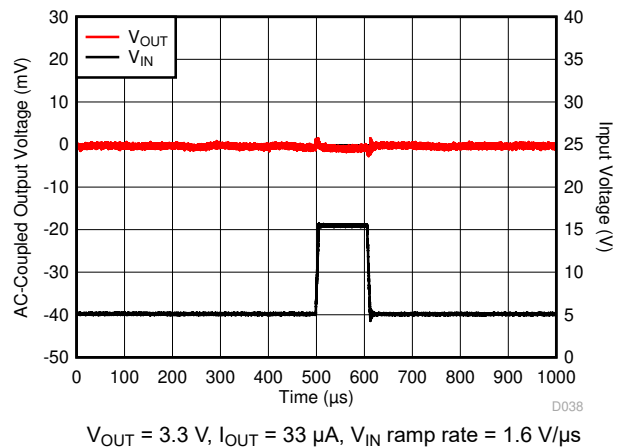
FIG 6-10. V_{IN} Transient From 5 V to 16 V
