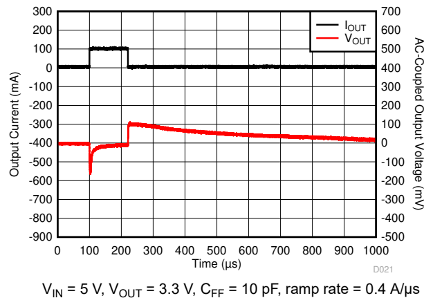
FIG 6-9. I_{OUT} Transient From 0 mA to 100 mA
