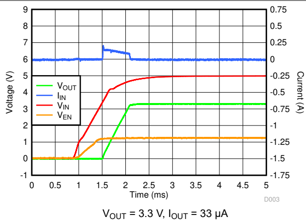
FIG 6-23. Startup Inrush Current With C_{OUT} = 22\text{ }\mu\text{F}
