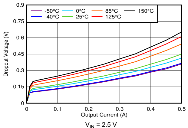
FIG 6-12. V_{DO} vs I_{OUT}
