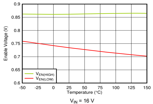
图 6-16. V_{EN} Thresholds vs Temperature
