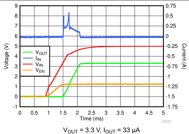
FIG 6-24. Startup Inrush Current With C_{OUT} = 47\text{ }\mu\text{F}
