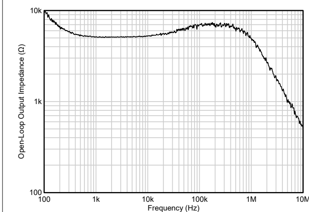
図 5-11. Open-Loop Output Impedance vs Frequency
