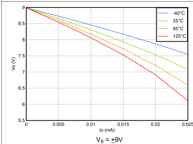
5-23. Output Voltage Swing vs Output Current (Sourcing)
