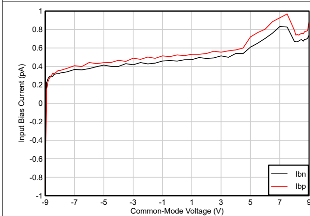
5-21. Input Bias Current vs Common-Mode Voltage
