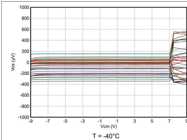
5-19. Input Offset Voltage vs Common-Mode Voltage
