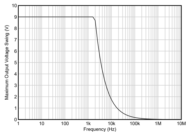
図 5-12. Maximum Output Voltage vs Frequency
