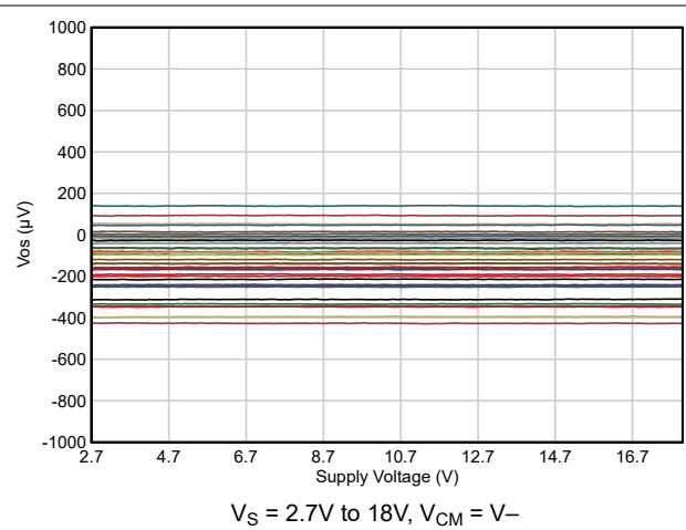
5-20. Input Offset Voltage vs Supply Voltage
