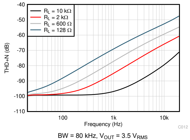
FIG 6-20. THD+N Ratio vs Frequency
