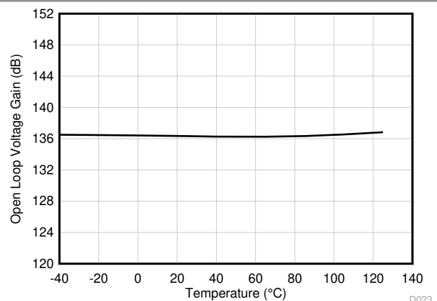
FIG 6-24. Open-Loop Voltage Gain vs Temperature (dB)
