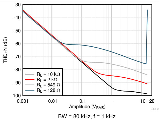
FIG 6-21. THD+N vs Output Amplitude
