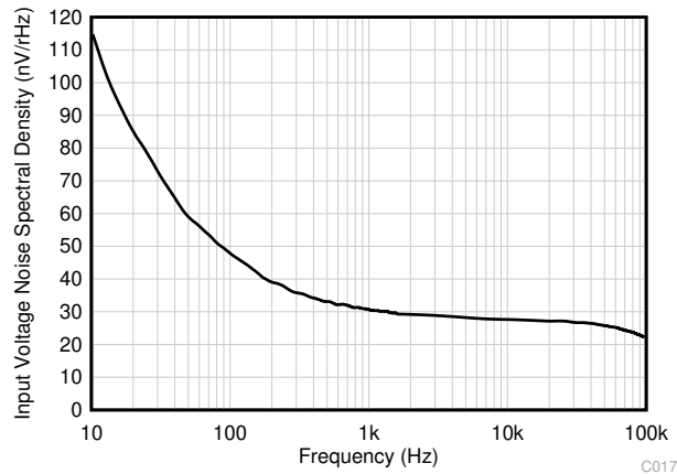
FIG 6-19. Input Voltage Noise Spectral Density vs Frequency
