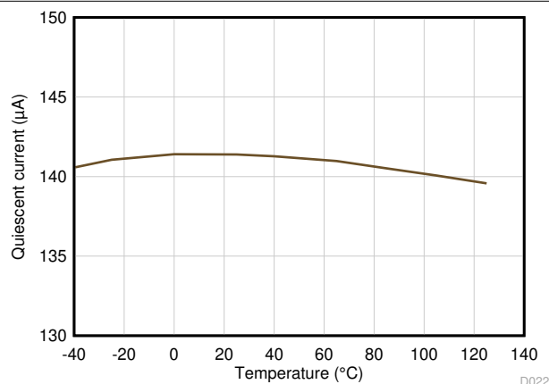
FIG 6-23. Quiescent Current vs Temperature
