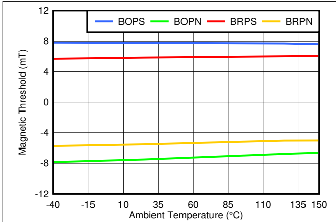
7-7. TMAG5123C Magnetic Thresholds vs. Temperature
