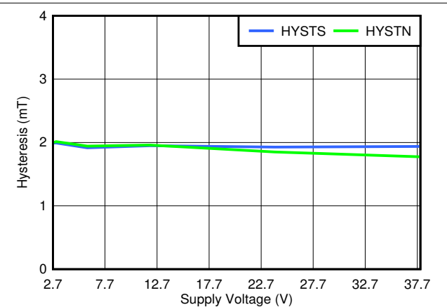
7-10. TMAG5123C Hysteresis vs. Supply Voltage
