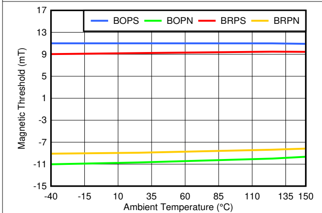
7-11. TMAG5123D Magnetic Thresholds vs. Temperature
