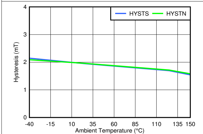
7-9. TMAG5123C Hysteresis vs. Temperature
