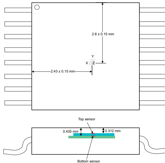
6-2. Location of X, Y, Z Hall Elements
