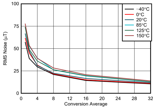
5-7. Z-Axis Noise vs Conversion Average, 100-mT Range
