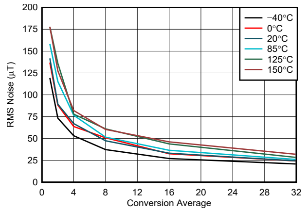
5-8. X, Y-Axis Noise vs Conversion Average, 100-mT Range
