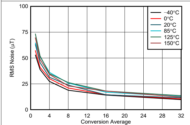
5-5. Z-Axis Input vs Conversion Average, 75-mT Range
