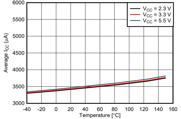
5-14. Active Mode Supply Current vs Temperature
