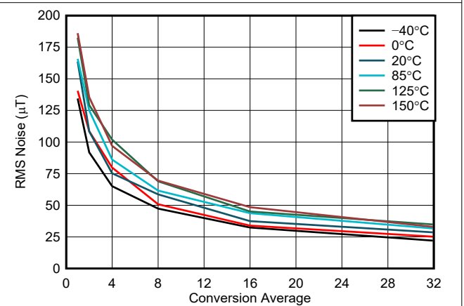
5-6. X, Y-Axis Noise vs Conversion Average, 75-mT Range
