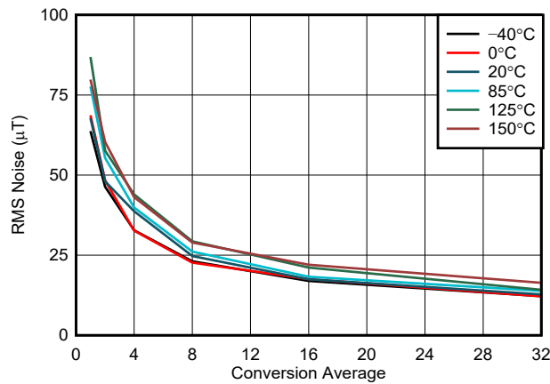
5-9. Z-Axis Noise vs Conversion Average, 150-mT Range
