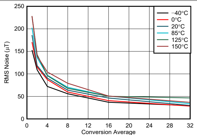
5-12. X, Y-Axis Noise vs Conversion Average, 300-mT Range
