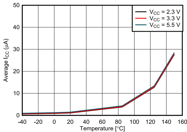
5-17. Sleep Mode Supply Current vs Temperature
