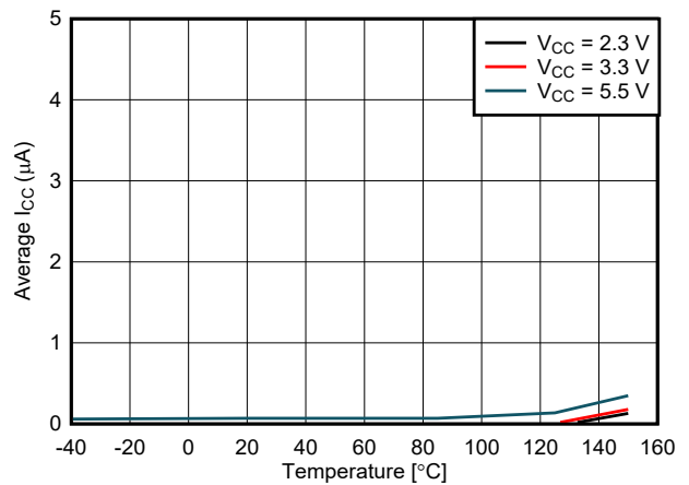
5-18. Deep Sleep Mode Supply Current vs Temperature
