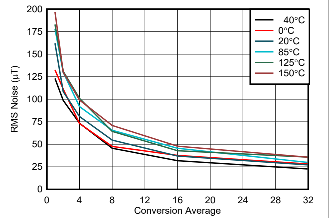
5-4. X, Y-Axis Noise vs Conversion Average, 50-mT Range
