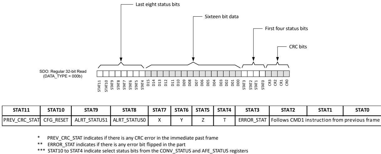
6-7. Regular 32-Bit SDO Read
