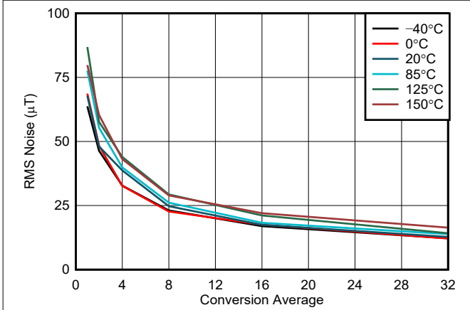
5-3. Z-Axis Noise vs Conversion Average, 50-mT Range
