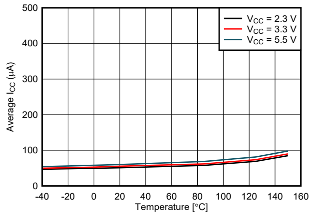
5-16. Configuration Mode Supply Current vs Temperature
