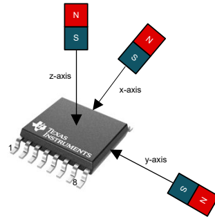
6-1. Direction of Applied Magnetic South Pole to Generate Positive ADC Codes
