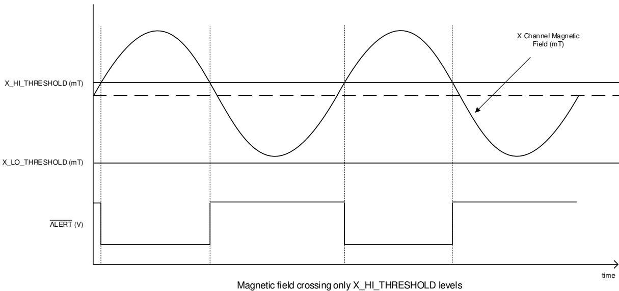
Figure 6-3. ALERT Pin Working as Magnetic Switch
