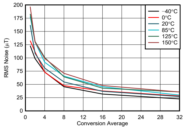
5-10. X, Y-Axis Noise vs Conversion Average, 150-mT Range
