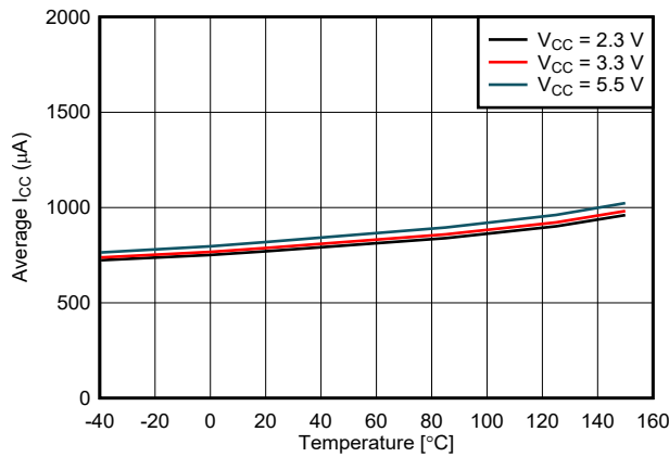
5-15. Standby Mode Supply Current vs Temperature
