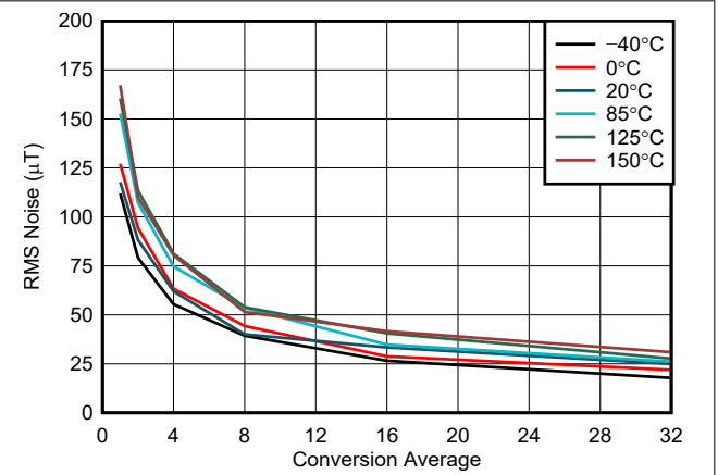
5-2. X, Y-Axis Noise vs Conversion Average, 25-mT Range
