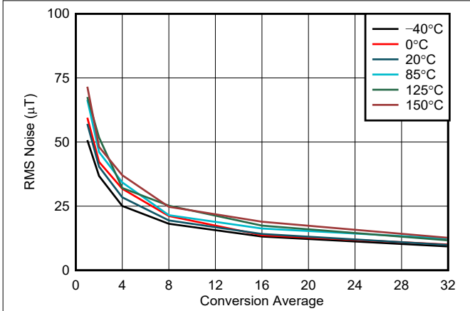
5-1. Z-Axis Noise vs Conversion Average, 25-mT Range
