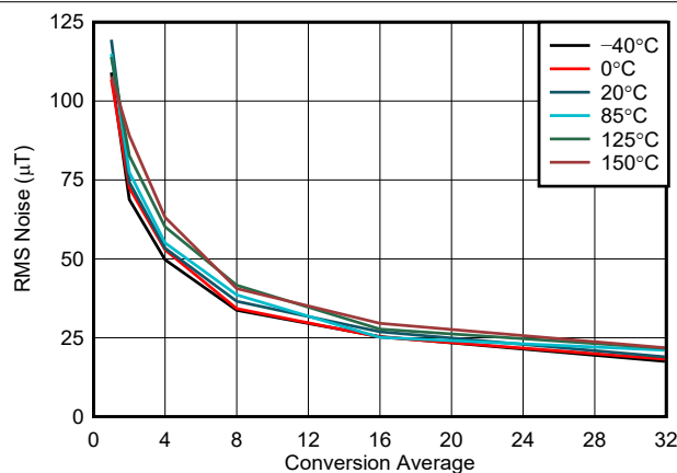
5-11. Z-Axis Noise vs Conversion Average, 300-mT Range
