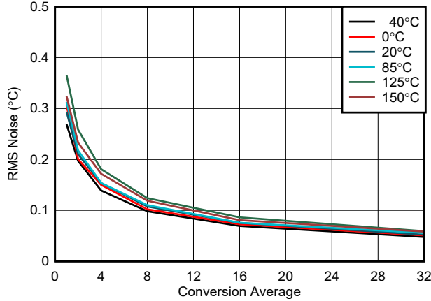
5-13. Temperature Sensor Noise vs Conversion Average
