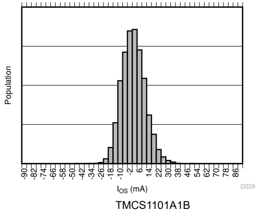
7-9. Input Offset Current Production Distribution
