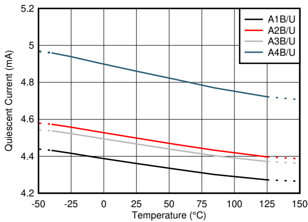
7-21. Quiescent Current vs. Temperature
