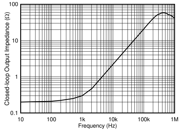
7-20. Output Impedance vs. Frequency
