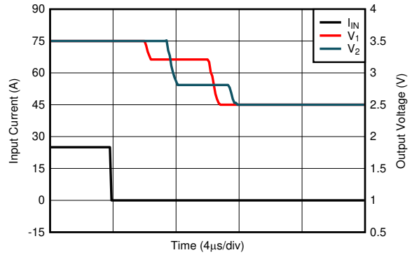
7-24. Voltage Output Step, Falling
