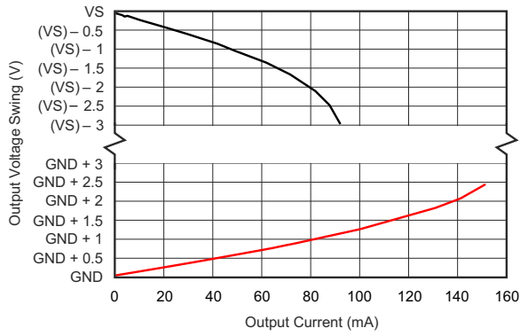
7-19. Output Swing vs. Output Current
