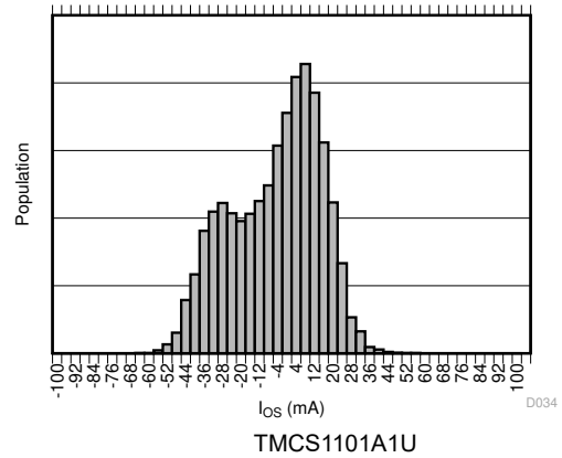
7-10. Input Offset Current Production Distribution
