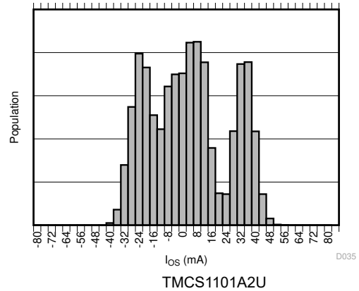
7-12. Input Offset Current Production Distribution
