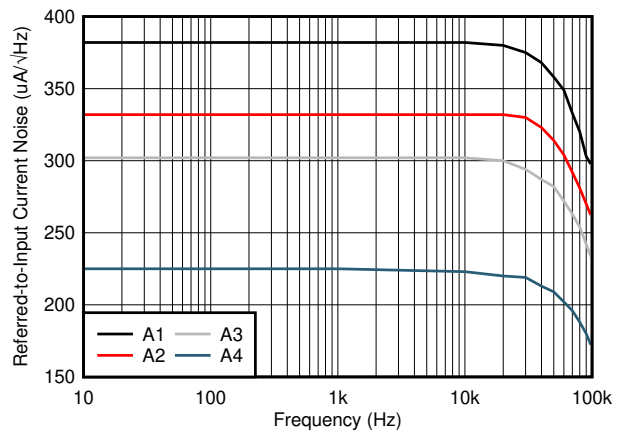
7-22. Input-Referred Noise vs. Frequency
