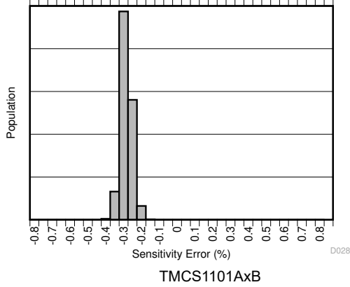
7-7. Sensitivity Error Production Distribution
