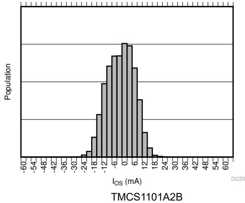
7-11. Input Offset Current Production Distribution
