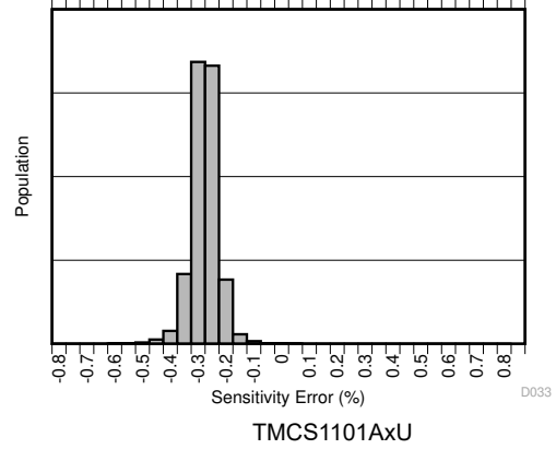
7-8. Sensitivity Error Production Distribution
