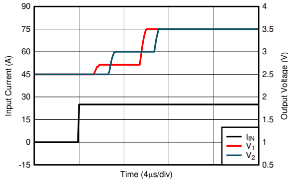
7-23. Voltage Output Step, Rising
