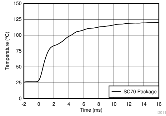
6-8. Thermal Response (Air-to-Fluid Bath)
