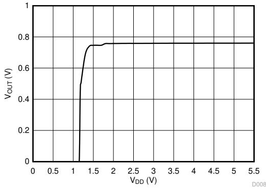
6-7. Output Voltage vs Power Supply
