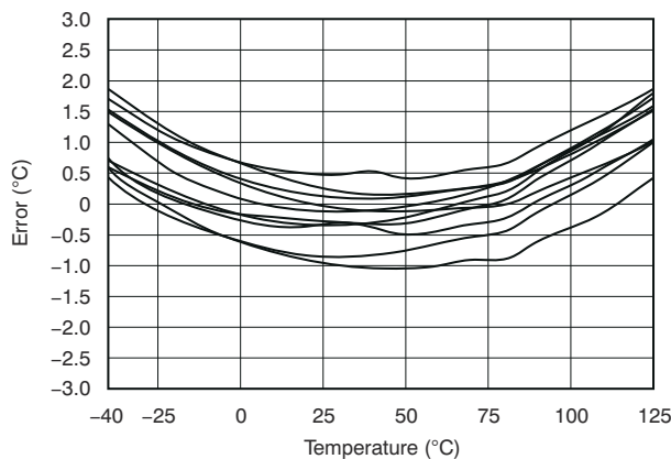
6-5. Typical Analog Output Error
