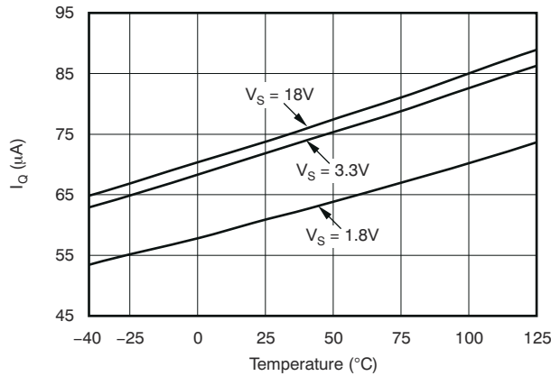
6-1. Quiescent Current Over Temperature and Supply
