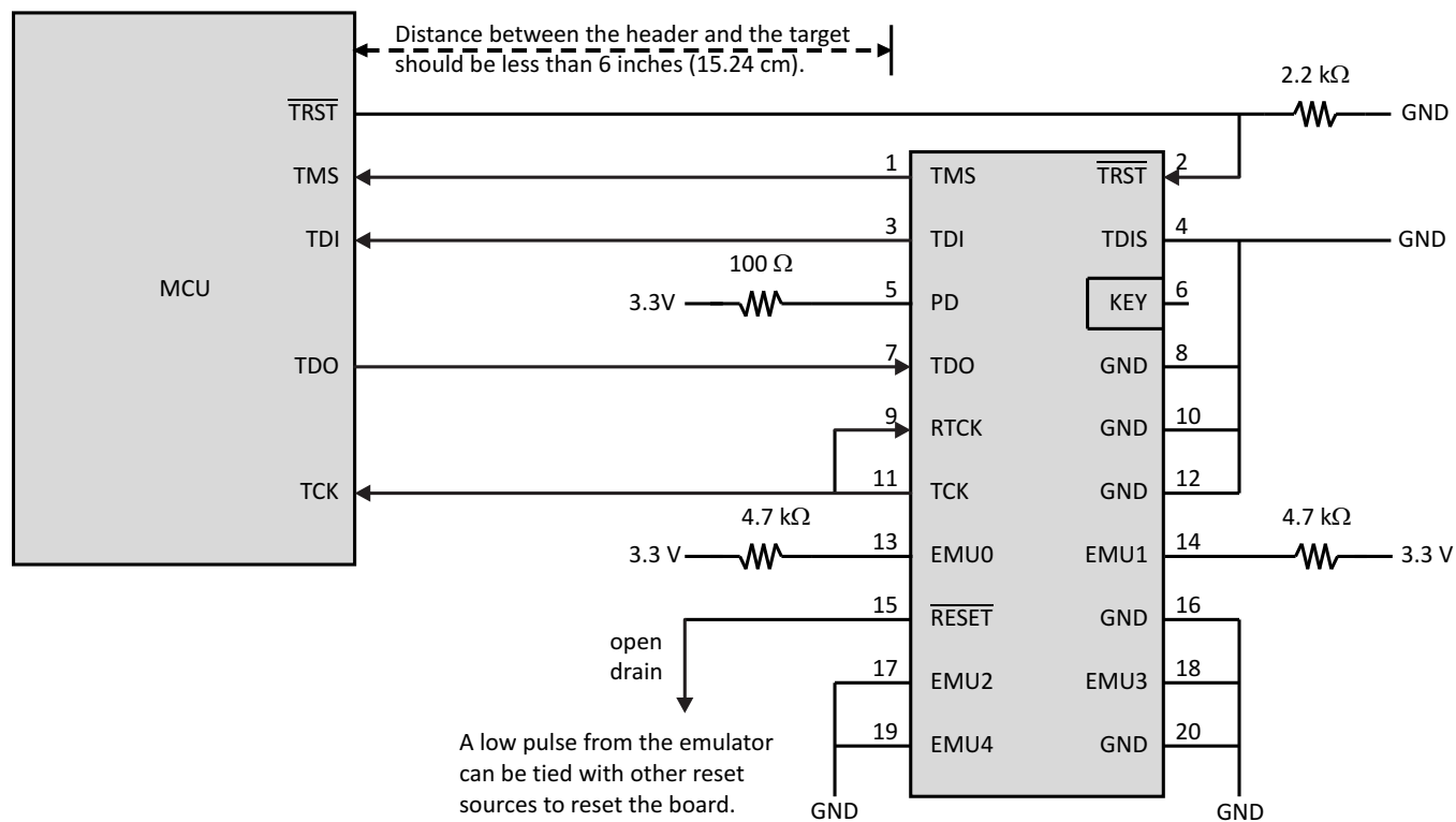
✎ 4-11. Connecting to the 20-Pin JTAG Header
