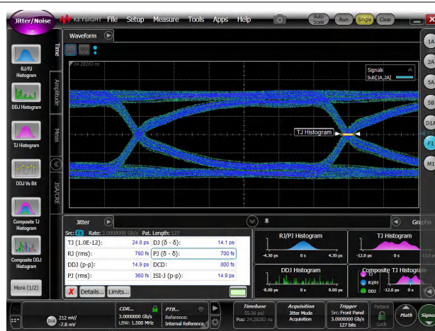
Figure 6-10. Through a Typical TMUXHS221LV Channel at 3Gbps
