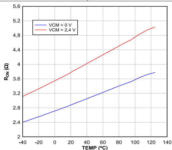
Figure 6-6. R_{ON} vs Ambient Temperature
