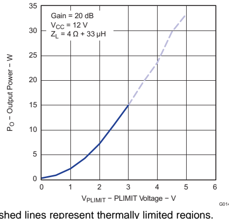
Figure 14. Output Power vs PLIMIT Voltage (BTL)
