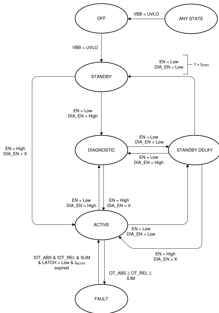
9-12. State Diagram
