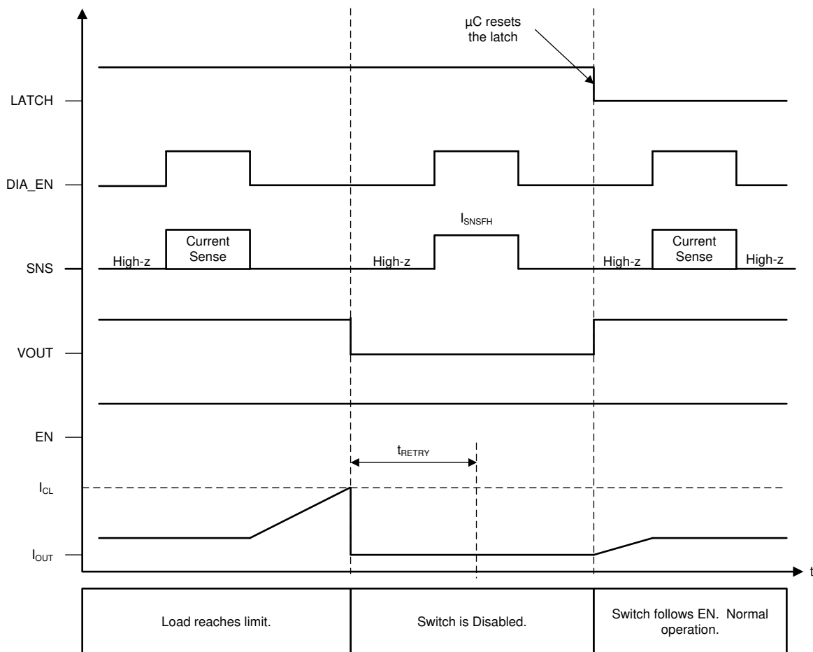
☒ 9-5. Current Limit – Version A and B - Latched Behavior
