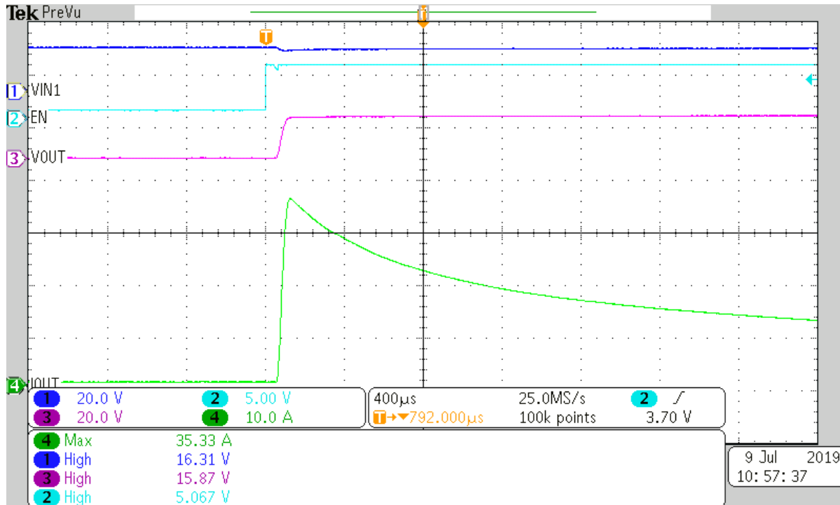
✎ 10-5. TPS1HB35-Q1 Version F 21W Bulb Inrush
