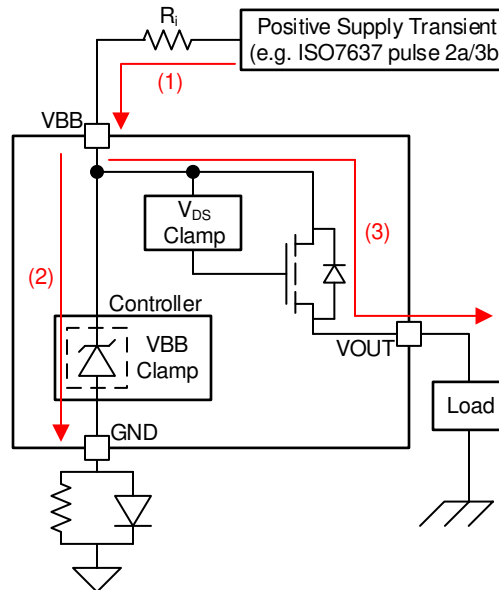
FIG 9-3. Current Path During Supply Voltage Transient
