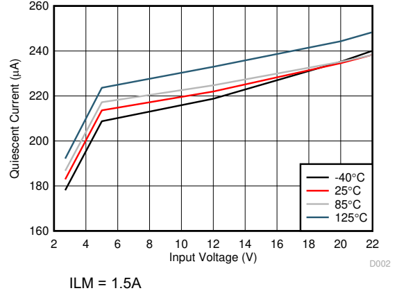
7-2. Quiescent Current vs Input Voltage
