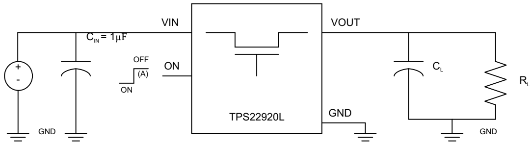
TEST CIRCUIT
