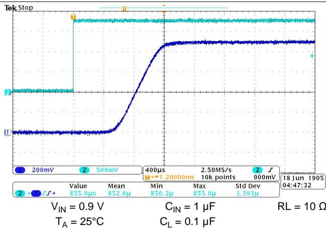
Figure 16. Turn-On Response
