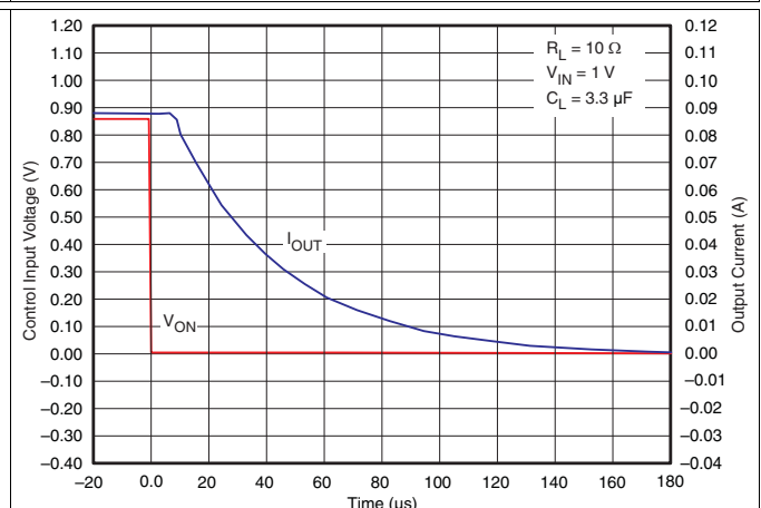
Figure 29. t_{OFF} Response
