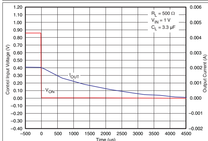
Figure 28. t_{OFF} Response
