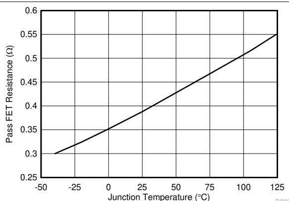
FIG 6-4. Pass FET Resistance vs Temperature
