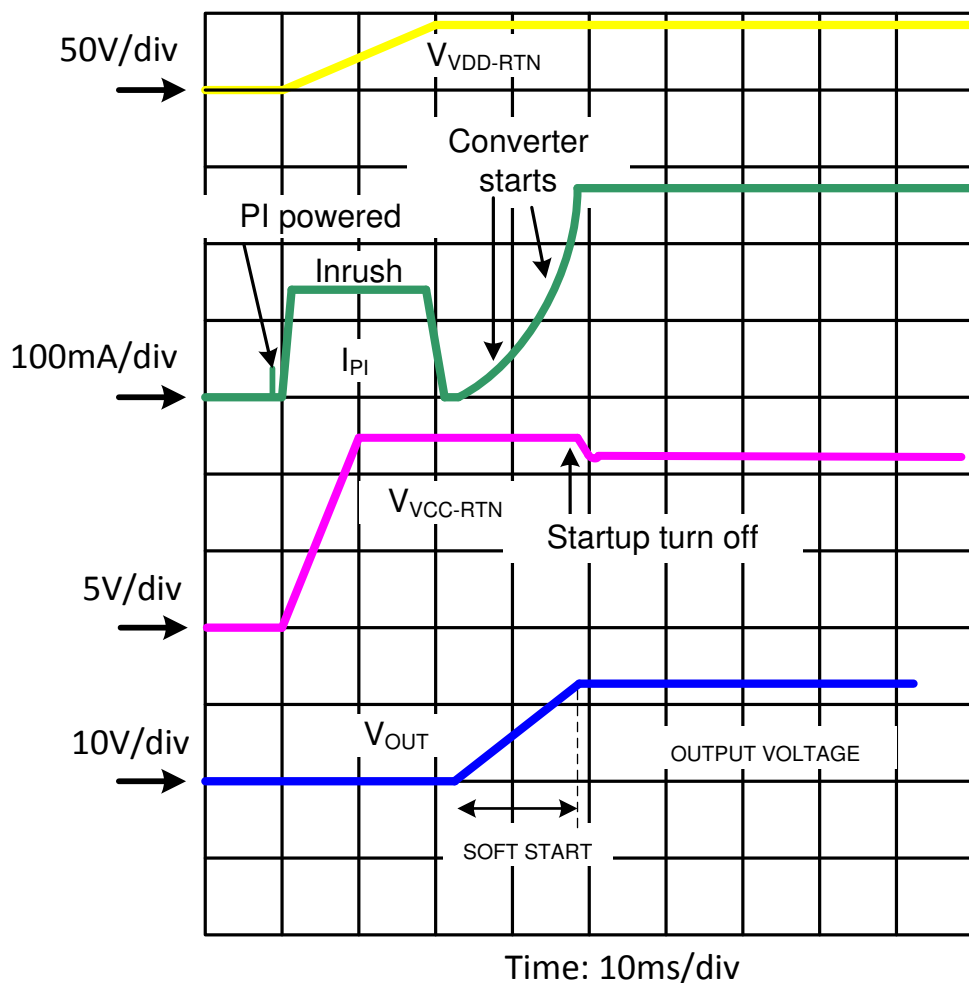
FIG 7-8. Power Up and Start
