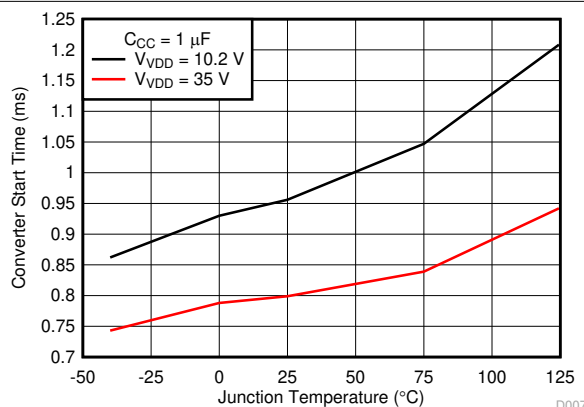
FIG 6-6. Converter Startup Time vs Temperature
