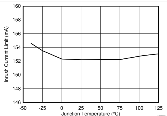
FIG 6-3. PoE Inrush Current Limit vs Temperature
