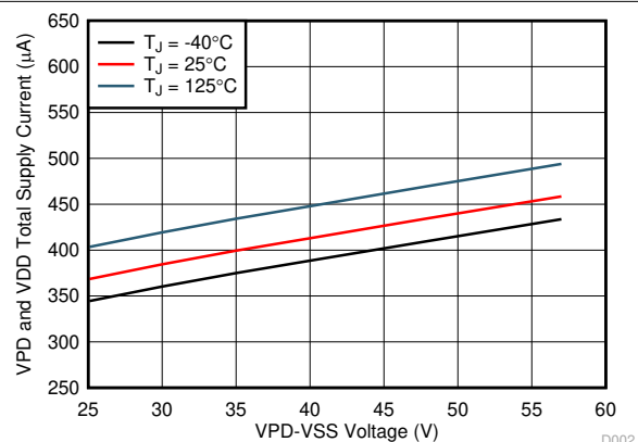
FIG 6-5. VPD and VDD Supply Current vs Voltage
