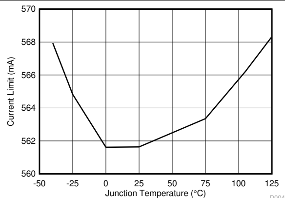
FIG 6-2. PoE Current Limit vs Temperature
