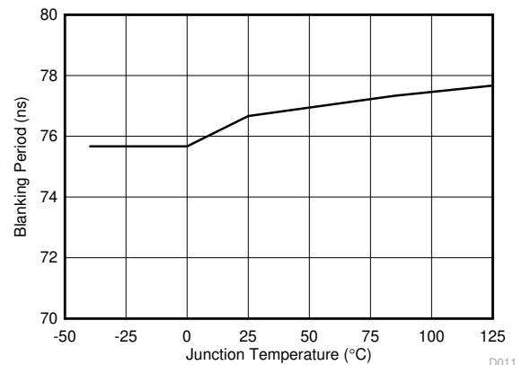
FIG 6-16. Blanking Period vs Temperature
