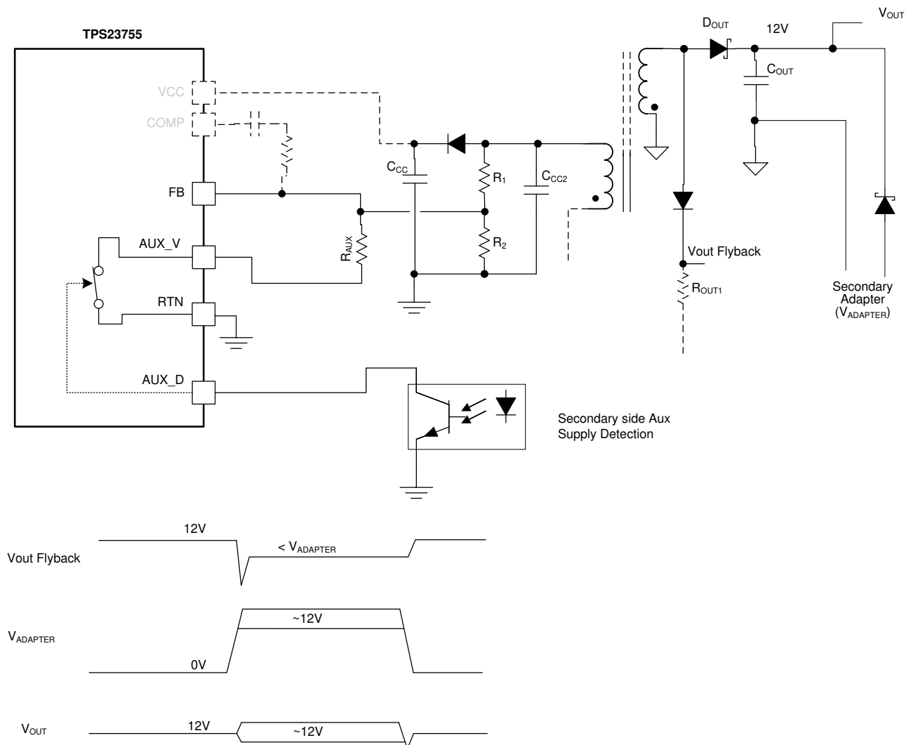
7-4. Secondary Side Priority Control with Smooth Transition
