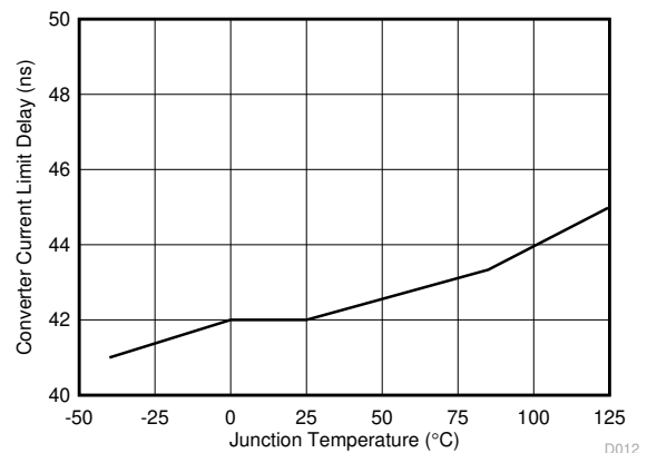
FIG 6-18. Converter Current Limit Delay vs Temperature
