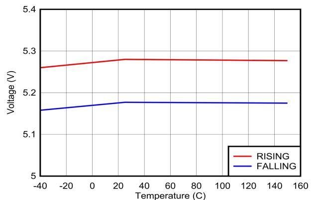
Figure 6-6. V_{IN}(\text{UVLO}) vs Temperature
