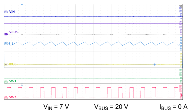
図 9-14. Boost Mode: Low V_{IN} , No Load
