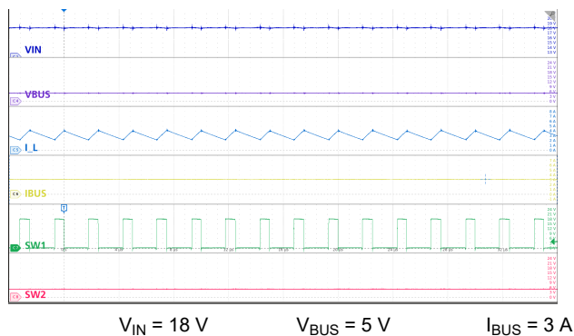
図 9-17. Buck Mode: High V_{IN} , 3 A load
