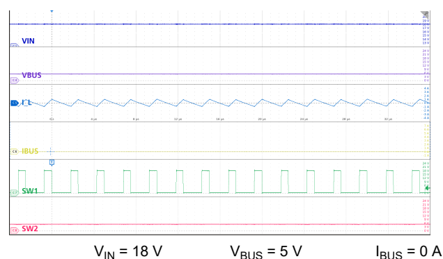
図 9-15. Buck Mode: High V_{IN} , No Load
