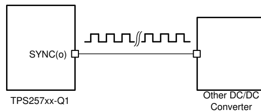
図 8-16. Using SYNC(o) to drive external DC/DC Converter
