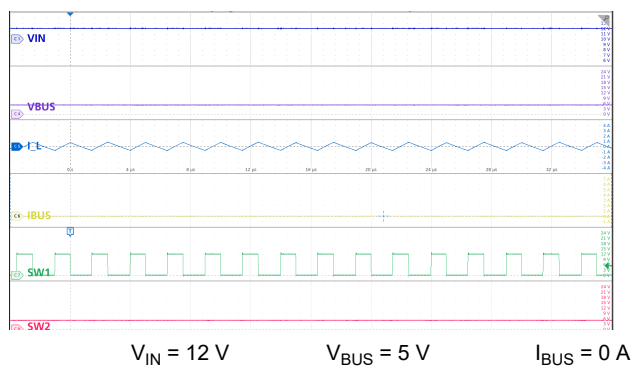
図 9-19. Buck Mode: Nominal V_{IN} , No Load
