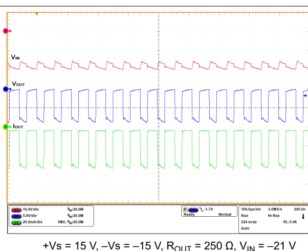
Figure 8-17. Thermal Protection During Loop Testing for I_{LOOP} < 0
