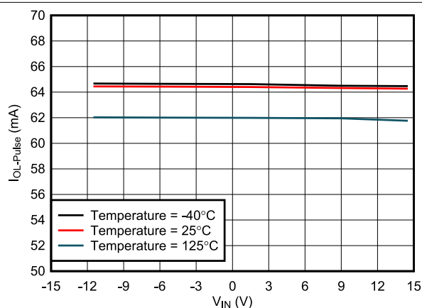
7-3. I_{OL} vs V_{IN} for I_{OUT} > 0
