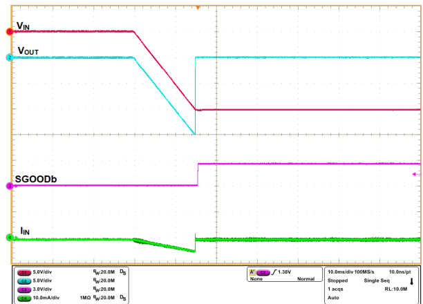
Figure 8-14. Input Undervoltage Protection
