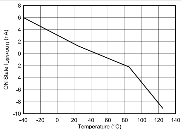
7-2. I_Q (IN+OUT) vs Temperature in Normal Operation
