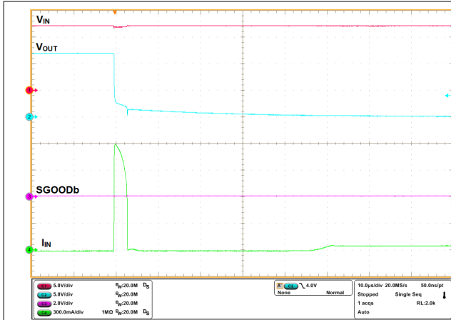
图 8-8. Fast-Trip Behavior
