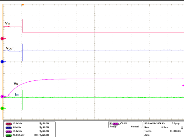
8-20. Transition to \pm V_s Supplies Power with R1 = 47 \text{ k}\Omega and R2 = 6.8 \text{ k}\Omega for supply Sensing
