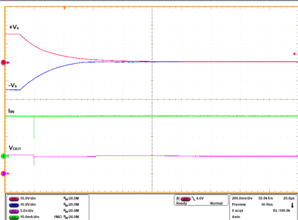
8-19. Transition to Loop Power With R1 = 47 \text{ k}\Omega and R2 = 6.8 \text{ k}\Omega for Supply Sensing
