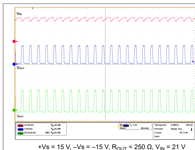
Figure 8-16. Thermal Protection During Loop Testing for I_{LOOP} > 0
