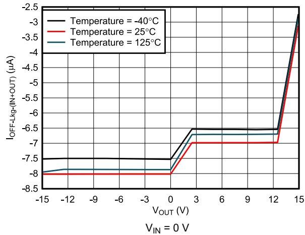
7-9. (I_{\text{OFF-Leakage-IN}} + I_{\text{OFF-Leakage-OUT}}) vs V_{\text{OUT}}
