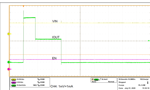
8-7. Current Limit Behavior for I_{OUT} > 2 \times I_{OL} with MODE = 180\text{ k}\Omega
