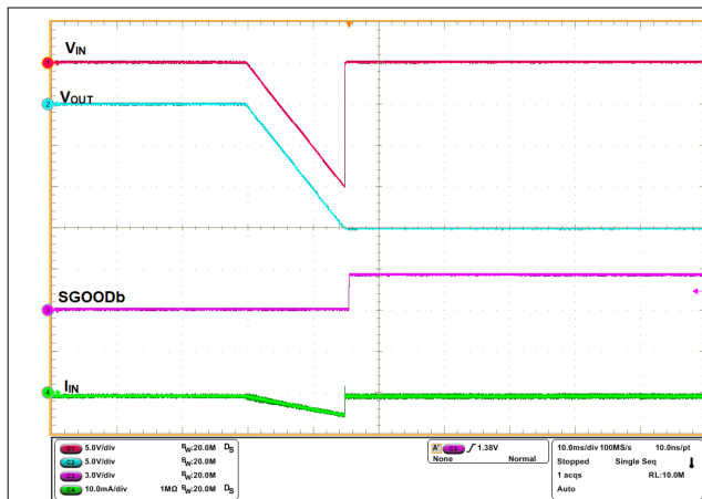
Figure 8-13. Output Undervoltage Protection
