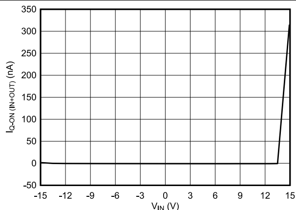
7-1. I_{Q-ON} (IN+OUT) vs V_{IN} in Normal Operation
