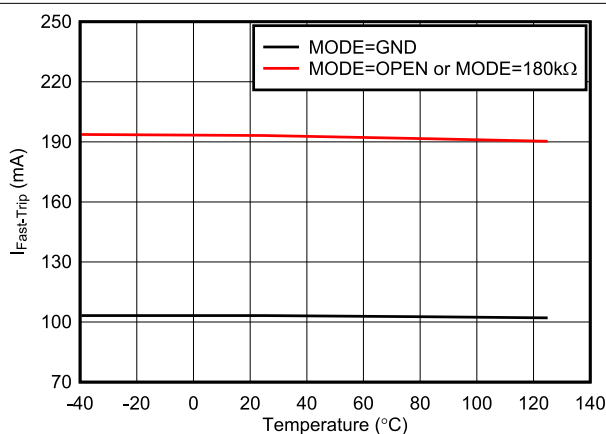
7-6. I_{Fast-Trip} vs Temperature for I_{OUT} > 0
