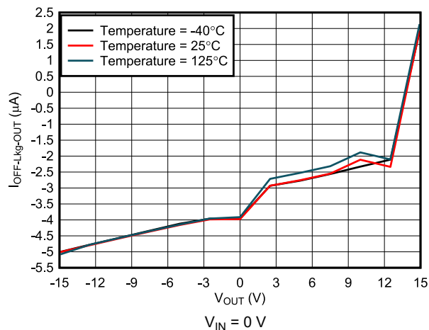
7-11. I_{\text{OFF-Leakage-OUT}} vs V_{\text{OUT}}
