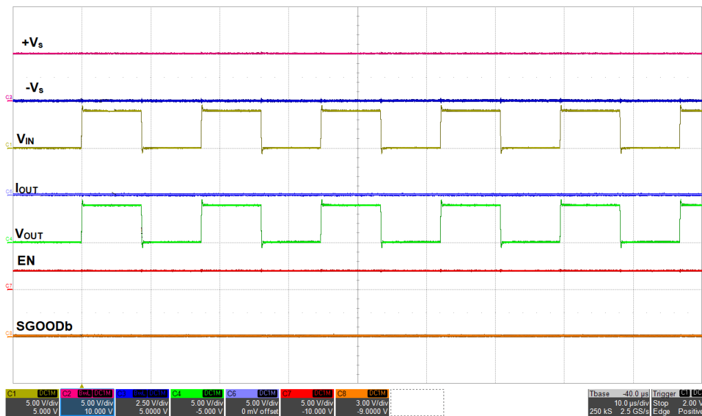
Figure 9-18. 115.2-Kbps UART Signal Through TPS2661x with V_s of 5 V
