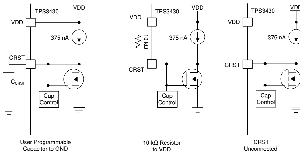
☒ 8-1. CRST Charging Circuit
