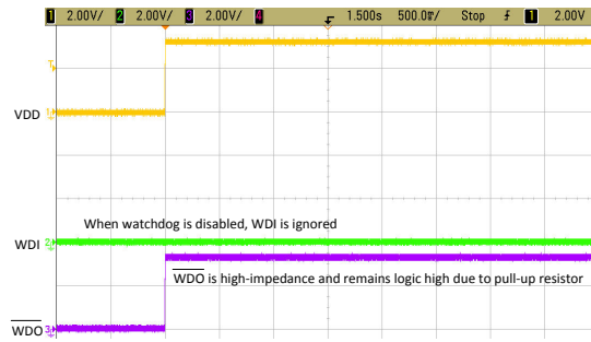
8-9. Watchdog Disabled With Missing WDI Pulse
