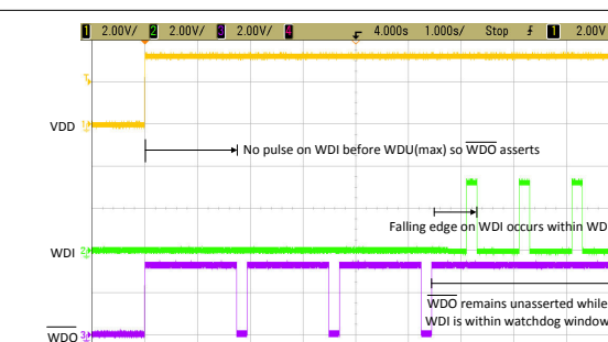
Figure 8-5. \overline{WDO} Fault Caused by missing WDI Pulses Followed by Correct Timing WDI Pulses
