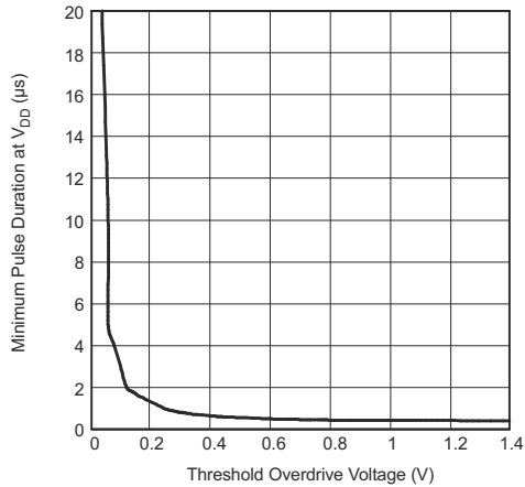
FIG 6-6. Minimum Pulse Duration At V DD vs V DD Threshold Overdrive Voltage
